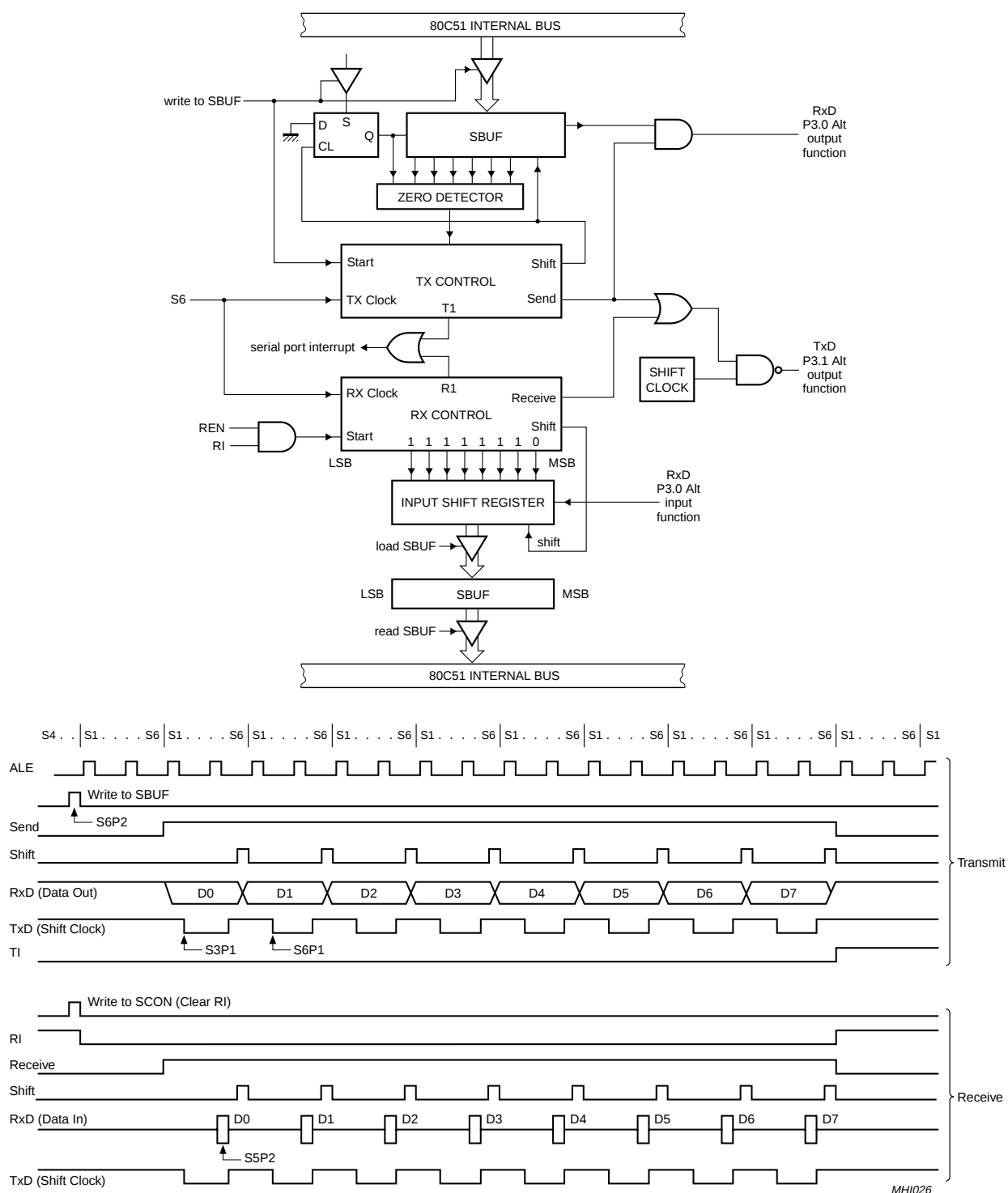
Fig.25 Serial Port Mode 0.
