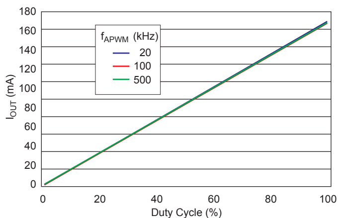
Figure 9. APWM pin dimming linearity.
