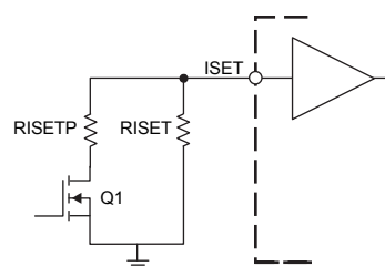
Figure 13. Configuration for 1000:1 dimming.
