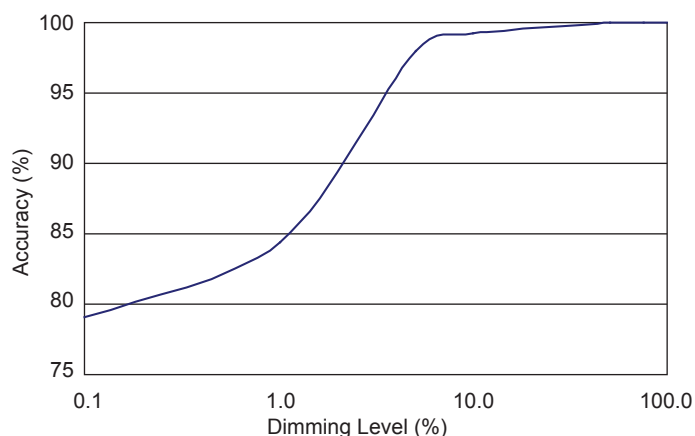
Figure 14. Typical accuracy, normalized to the 100% current level, versus dimming level, with F_{PWM} = 100 Hz.
