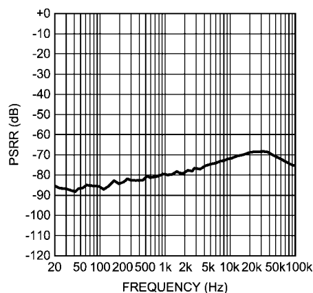
Loudspeaker PSRR vs Frequency LS\_V_{DD} = 3.3V , Aux Gain = 0dB Differential Aux Input to Ground V_{RIPPLE} = 200mV_{PP}
