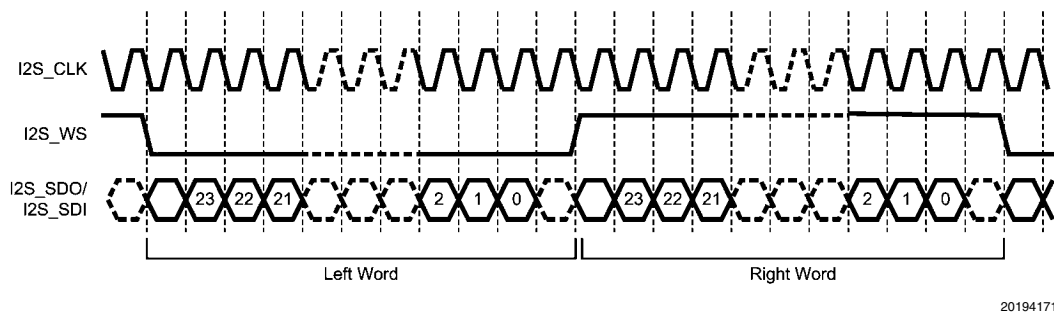
FIGURE 17. I²S Serial Data Format (24 bit example)
