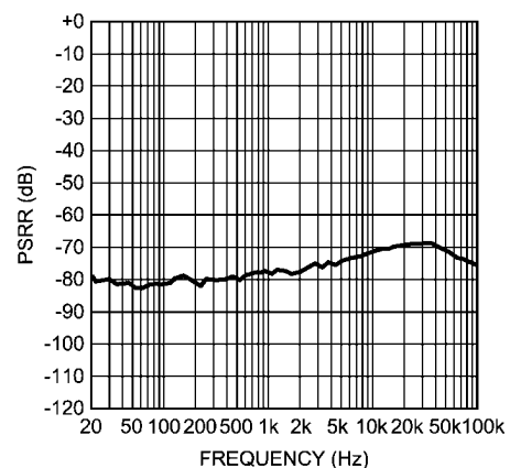
Loudspeaker PSRR vs Frequency LS\_V_{DD} = 4.2V , Aux Gain = 0dB Differential Aux Input to Ground V_{RIPPLE} = 200mV_{PP}
