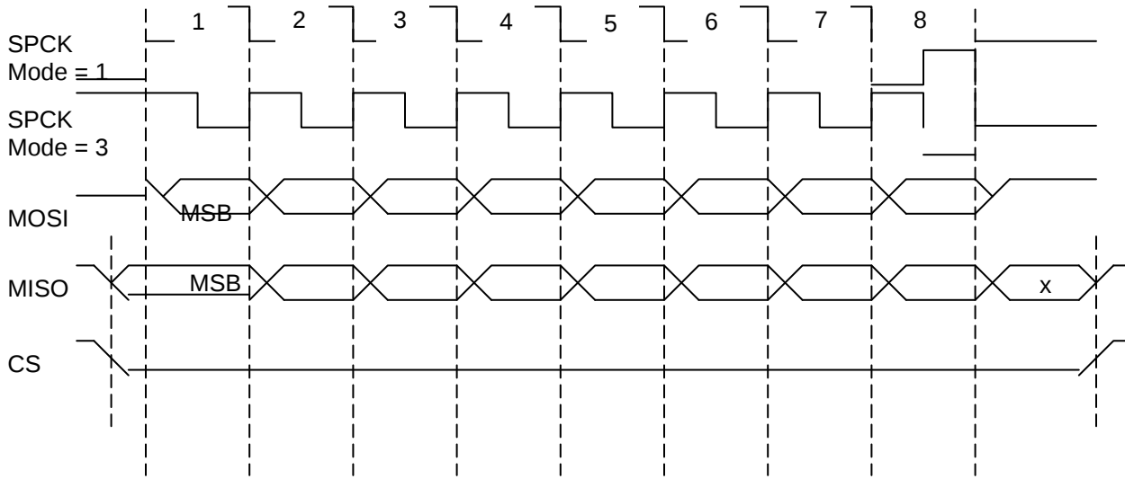
Figure 1. SPI Transfer Format (CKPHA=1, 8 bits per transfer)
