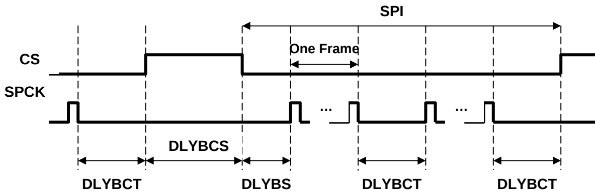
Figure 3. Programmable Delays
