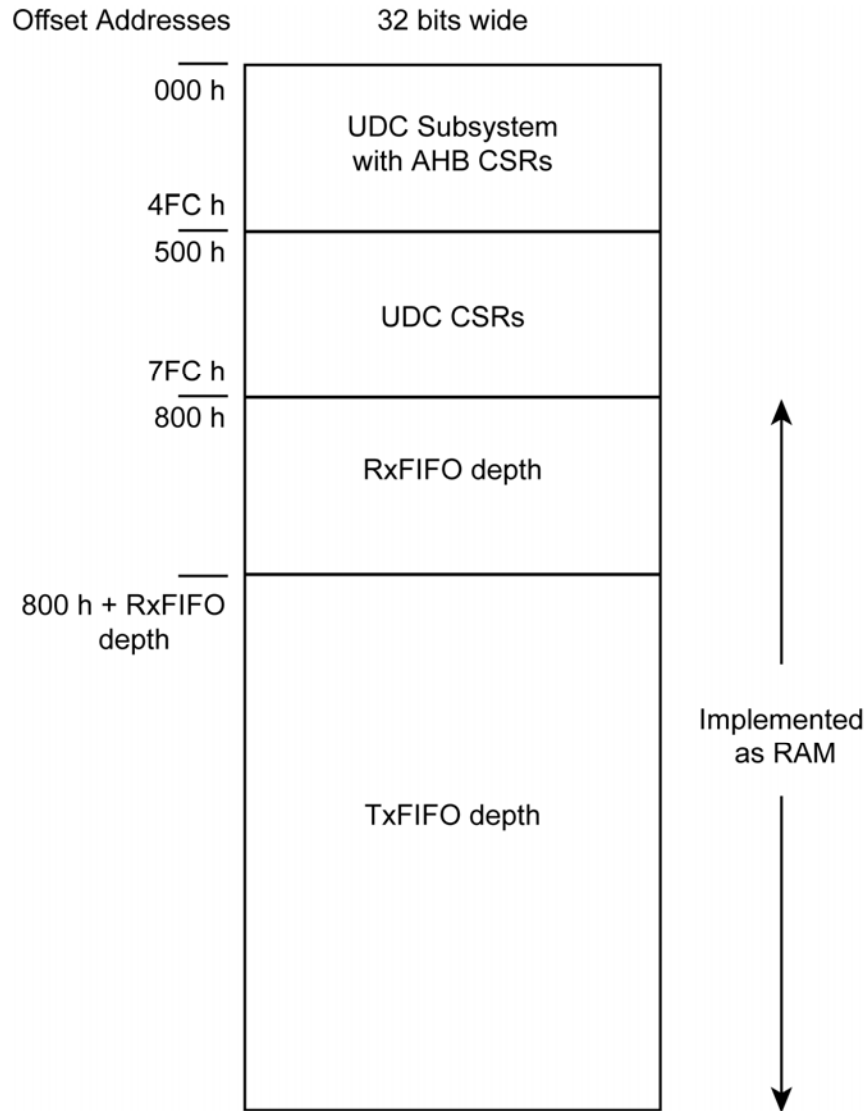
Memory Map (from processor viewpoint)
