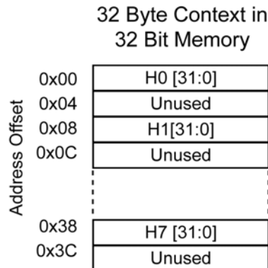
Hashing Context Memory Format
