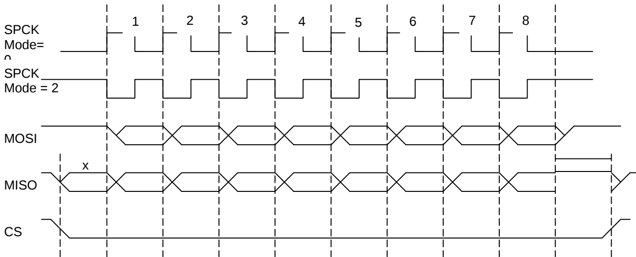
Figure 2. SPI Transfer Format (CKPHA=0, 8 bits per transfer)
