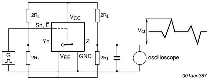
Figure 18. Test circuit for measuring crosstalk between control input and any switch
