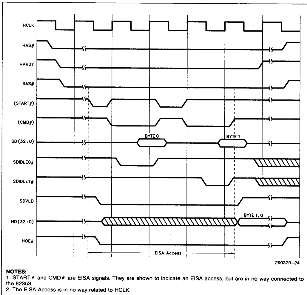
Figure 6.14. Host Single Read of System (16-Bit Slave)
