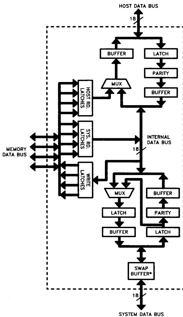
Figure 1.1. 82353 Internal Block Diagram
