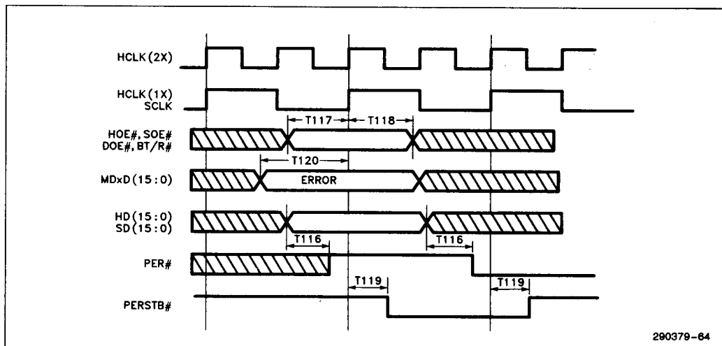
Figure 7.18. Parity Error Timing
