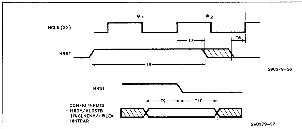
Figure 7.3. Reset Waveforms
