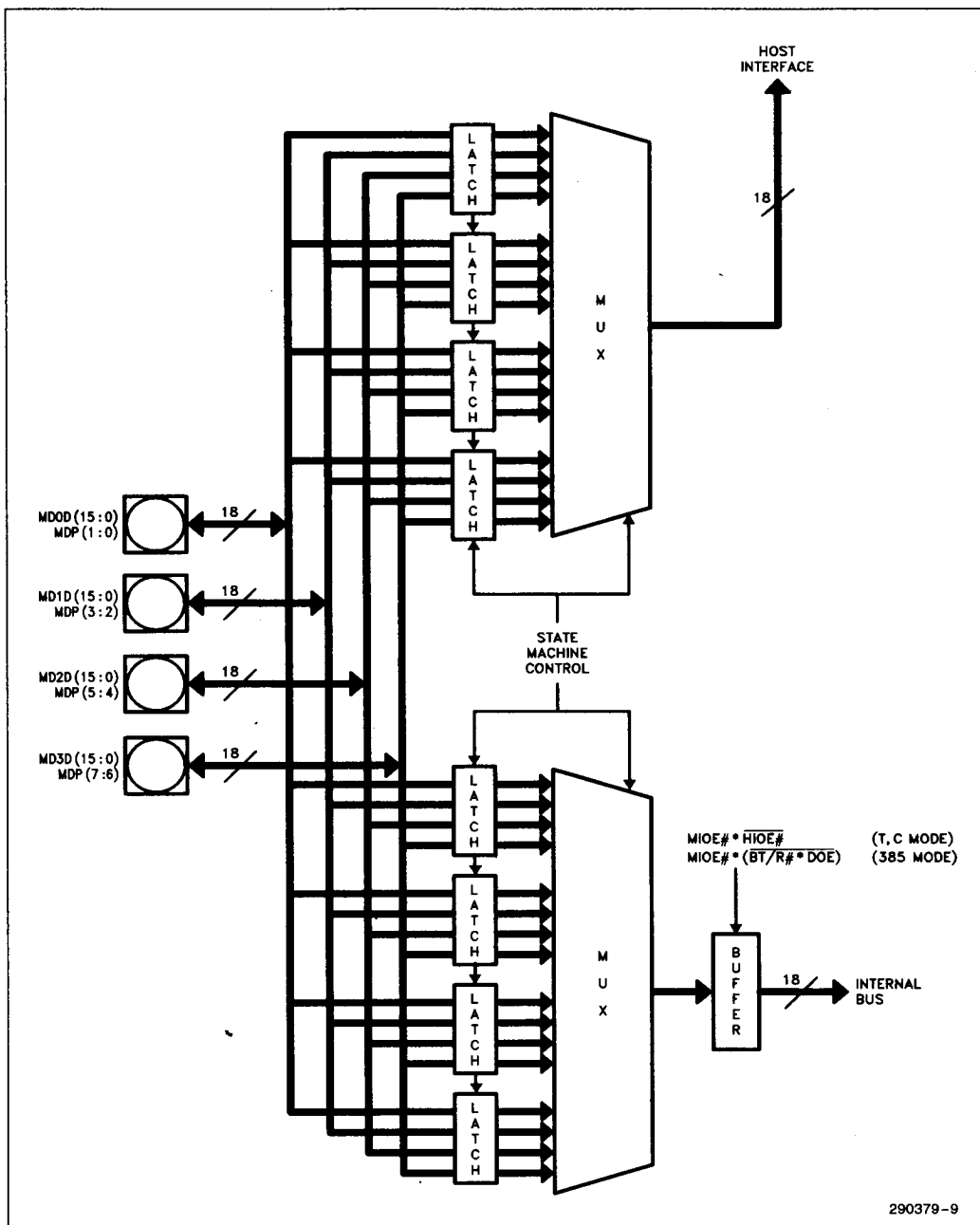
Figure 4.8. Memory Read Interface
