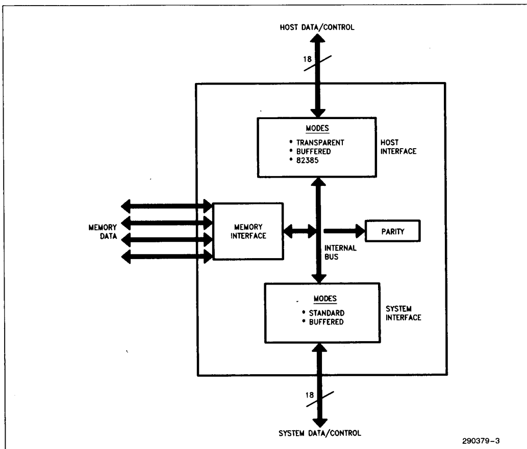
Figure 4.1. 82353 Functional Blocks
