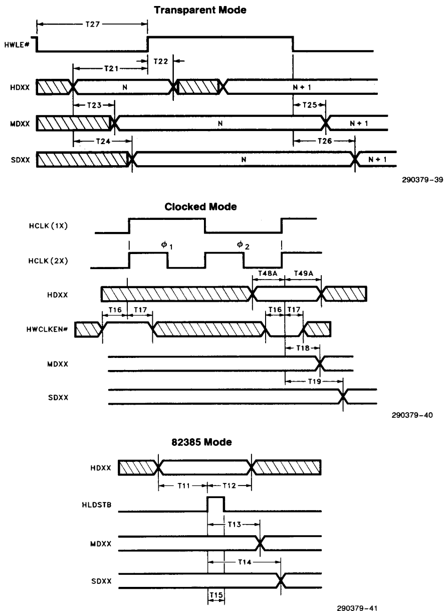
Figure 7.5. Host Latch Control
