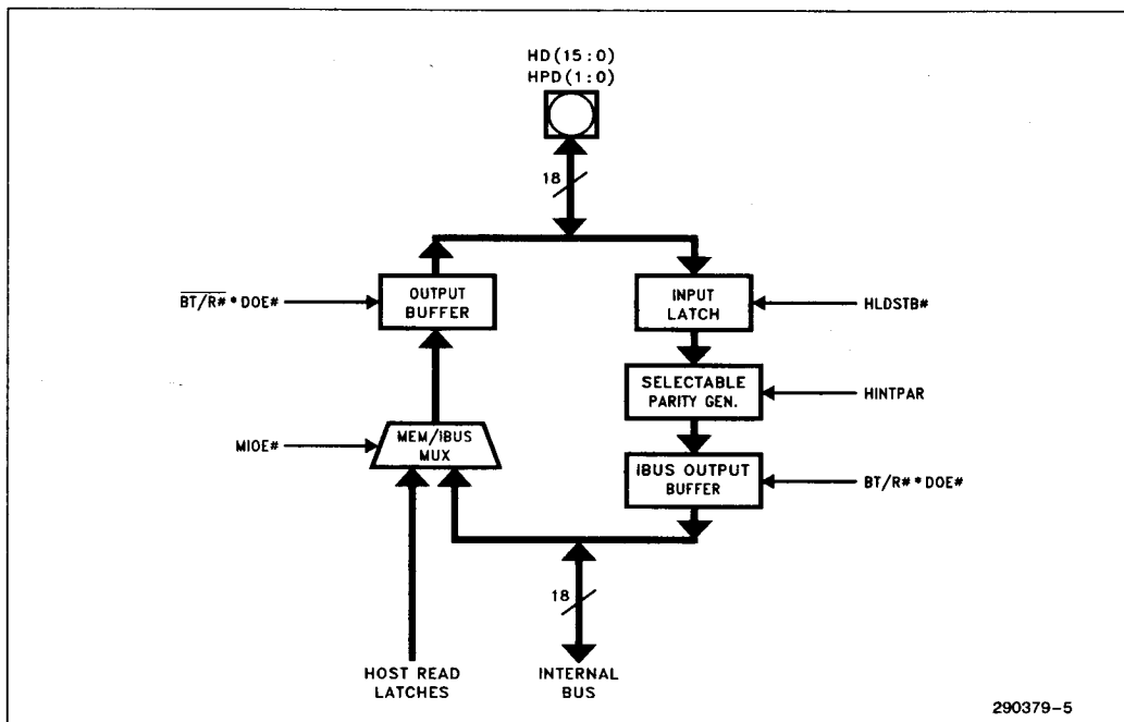
Figure 4.4. 82385 Host Mode
