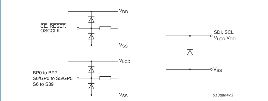
Fig 42. Device protection diagram for PCF8536BT
