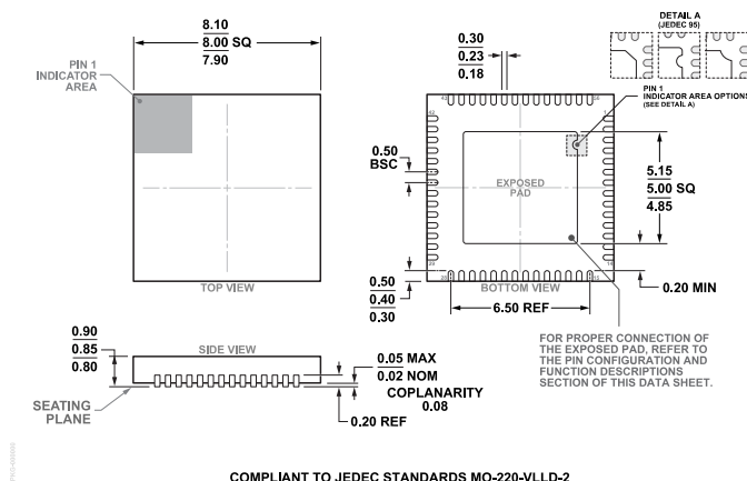
Figure 53. 56-Lead Lead Frame Chip Scale Package [LFCSP] 8 mm x 8 mm Body and 0.85 mm Package Height (CP-56-21) Dimensions shown in millimeters
