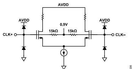
Figure 33. Clock Inputs
