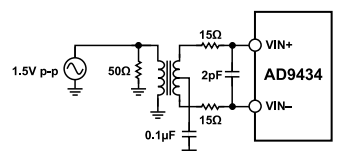
Figure 42. Differential Transformer—Coupled Configuration
