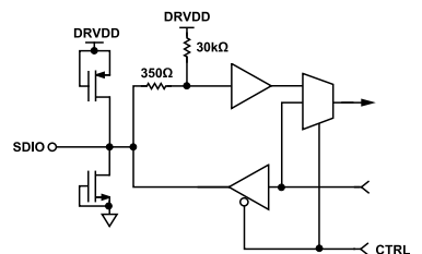
Figure 40. Equivalent SDIO Input Circuit
