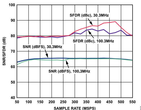
Figure 17. AD9434-500 SNR/SFDR vs. Sample Rate; 30.3 MHz, 100.3 MHz
