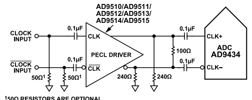
Figure 45. Differential PECL Sample Clock
