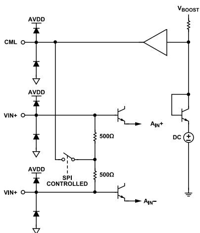
Figure 34. Analog Input DC Equivalent Circuit ( V_{CML} \approx 1.7\text{ V} )
