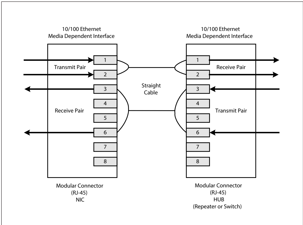
FIGURE 2-1: TYPICAL STRAIGHT CABLE CONNECTION
