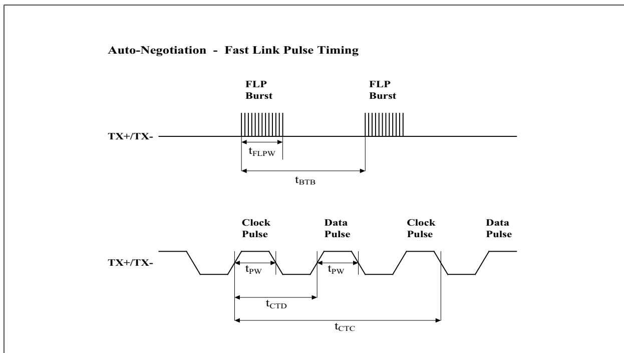
FIGURE 6-13: AUTO-NEGOTIATION TIMING
