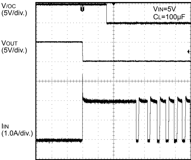
TIME(4ms/div.) Figure 37. Over-Current Response 1ΩLoad Connected at Enable
