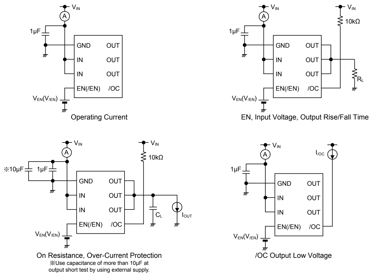
Figure 4. Measurement Circuit
