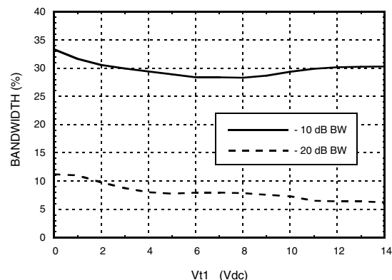
Rejection Bandwidth Vs. V_{t1}
