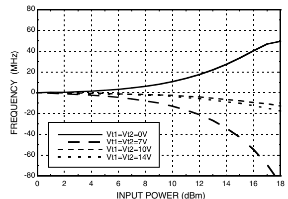
Rejection Band, Fcenter vs. Pin
