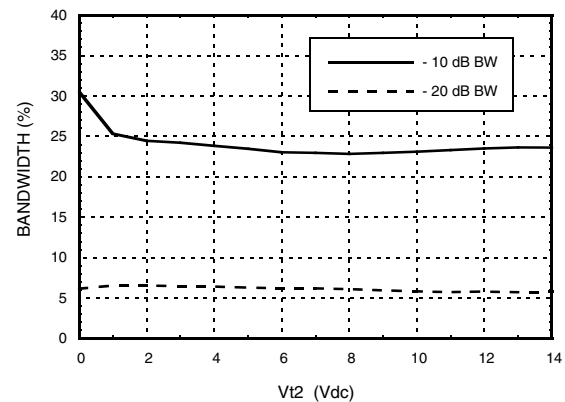
Rejection Bandwidth Vs. V_{t2}
