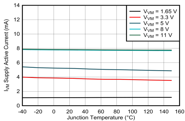
Figure 7-20. Active Current ( I_{VM} ) vs. Junction Temperature ( T_J )
