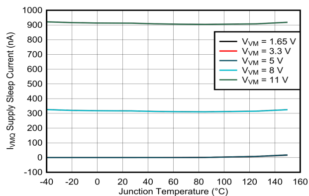
Figure 7-18. Sleep Current ( I_{VMQ} ) vs. Junction Temperature ( T_J )
