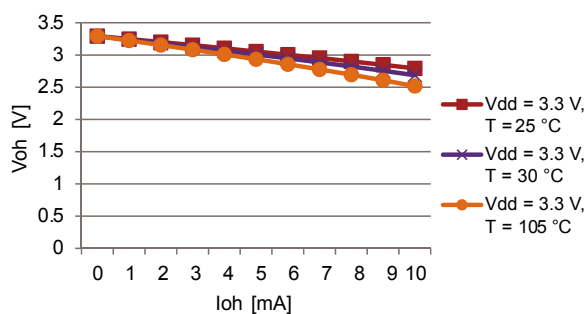
Figure 9. Standard pad @3.3 V, Vol
