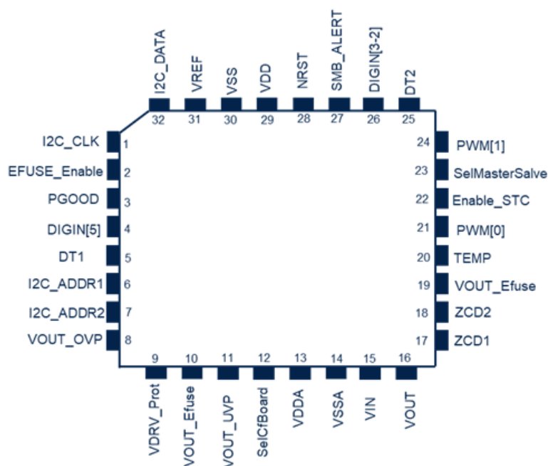
Figure 3. STNRG328S pinout
