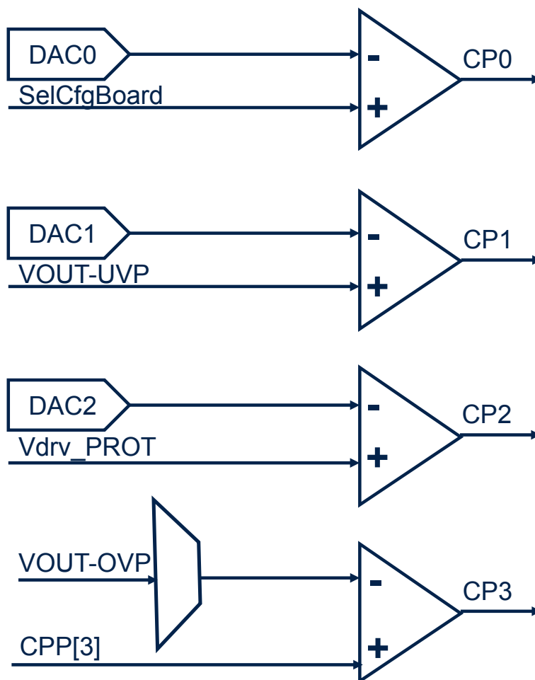
Figure 18. Analog Comparators
