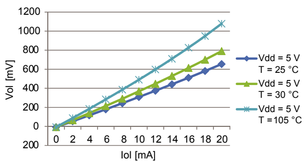
Figure 14. Fast pad @5 V, Voh
