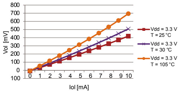
Figure 12. Fast pad @3.3 V, Voh
