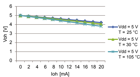
Figure 11. Standard pad @5 V, Vol
