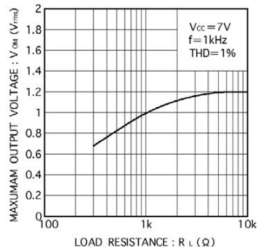
Fig.13 Maximum output voltage vs. load resistance
