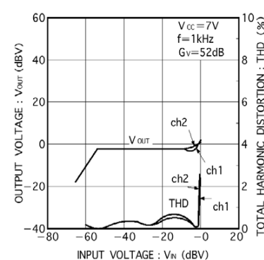
Fig.10 ALC characteristics
