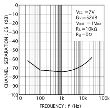
Fig.9 Channel separation vs. frequency
