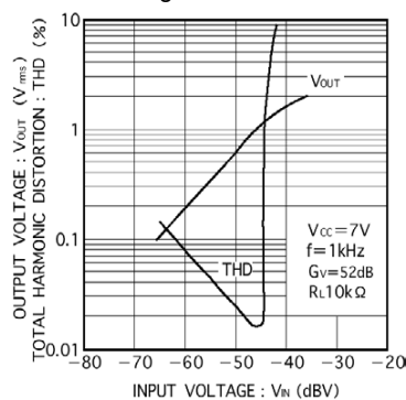
Fig.11 Input/output characteristics
