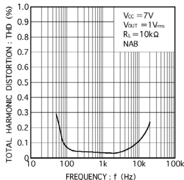
Fig.5 Total harmonic distortion vs. frequency
