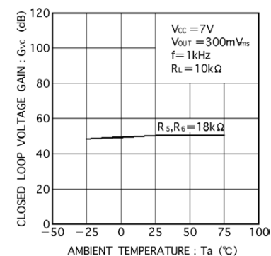
Fig.7 Closed loop voltage gain vs. ambient temperature
