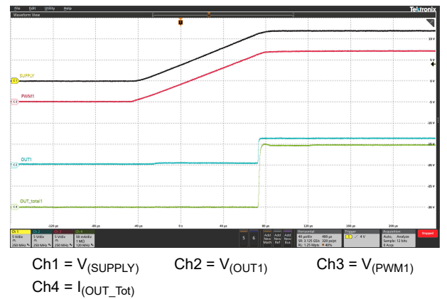
Figure 6-10. Power-Up Sequence
