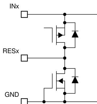
Figure 7-12. RESx Pins
