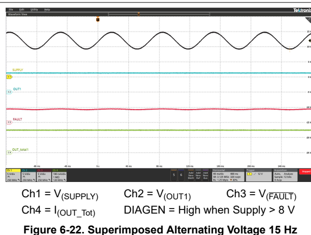
Figure 6-22. Superimposed Alternating Voltage 15 Hz
