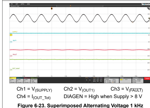
Figure 6-23. Superimposed Alternating Voltage 1 kHz
