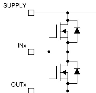
Figure 7-13. INx Pins
