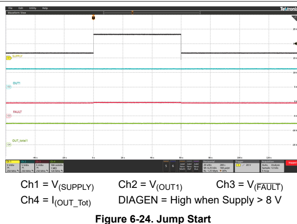
Figure 6-24. Jump Start
