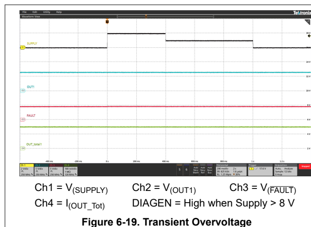
Figure 6-19. Transient Overvoltage
