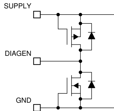
Figure 7-9. DIAGEN Pin
