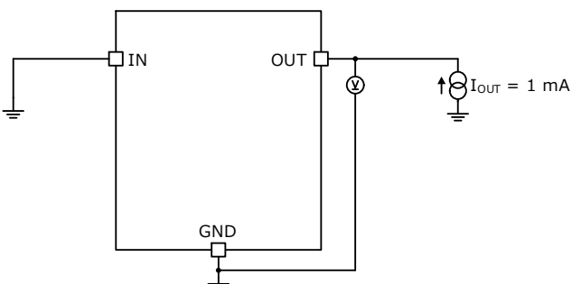
Measurement Circuit for Figure 8
