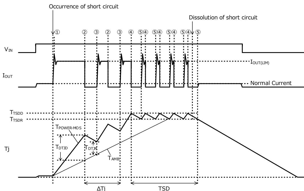
Figure 20. The Behavior when the OUT Pin Short Circuit
