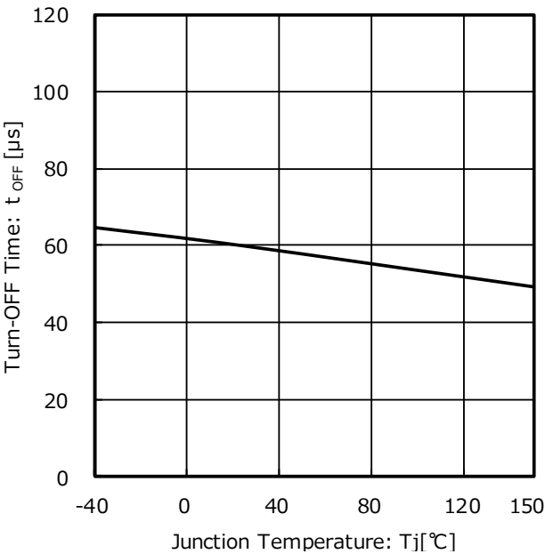
Figure 12. Turn-OFF Time vs Junction Temperature
