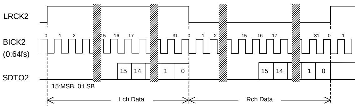
Figure 33. Mode 0 Timing
