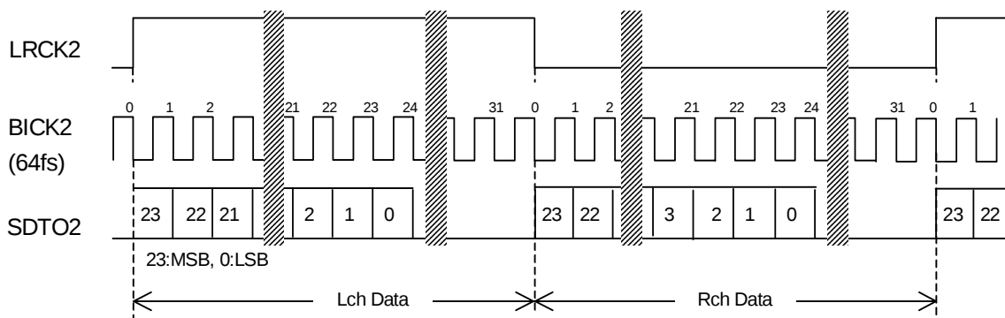
Figure 35. Mode 4, 6 Timing
