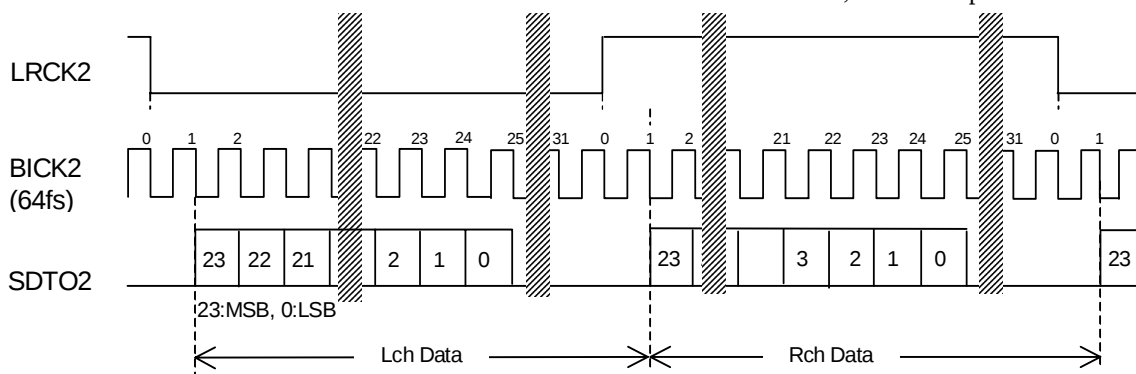
Figure 36. Mode 5, 7 Timing
