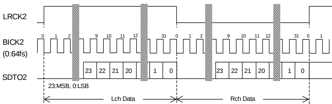
Figure 34. Mode 3 Timing
