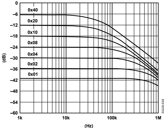
Figure 18. 100 k \Omega Gain vs. Frequency vs. Code
