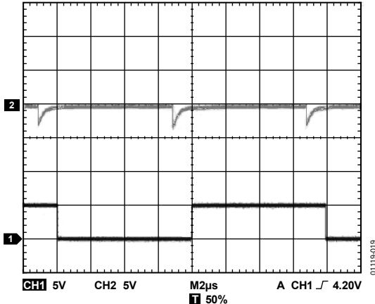
Figure 19. Midscale to Midscale – 1 Transition Glitch
