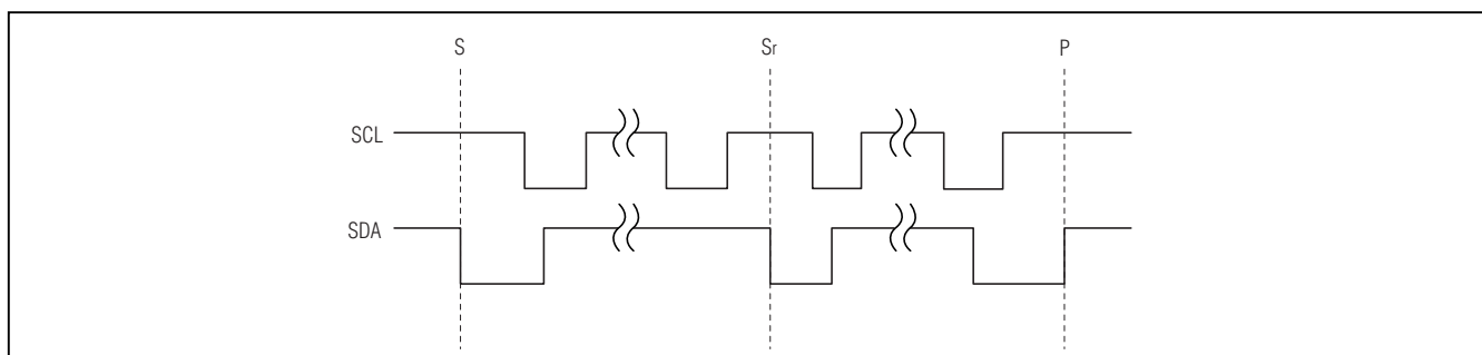
Figure 2. START/STOP Conditions
