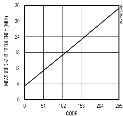
-3dB FREQUENCY vs. CONTROL CODE
