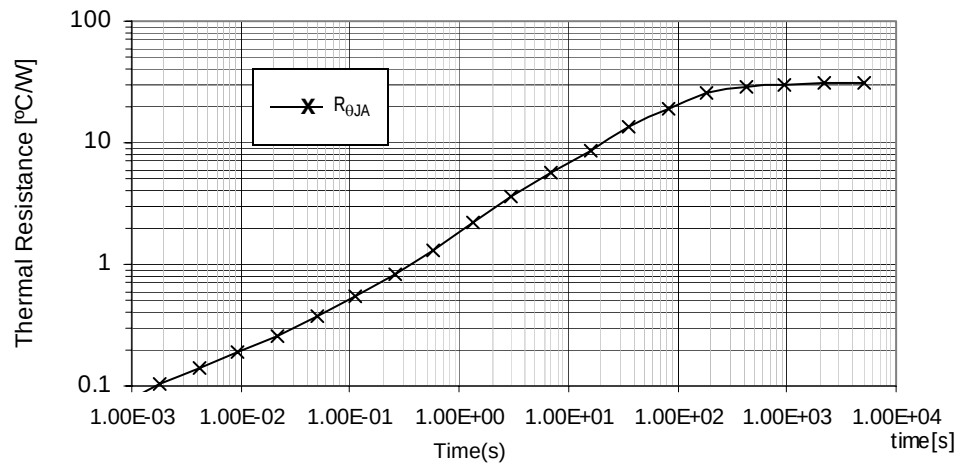
Figure 27. Transient Thermal Resistance R_{\theta JA} Device on Thermal Test Board Area A = 600 (mm²)
