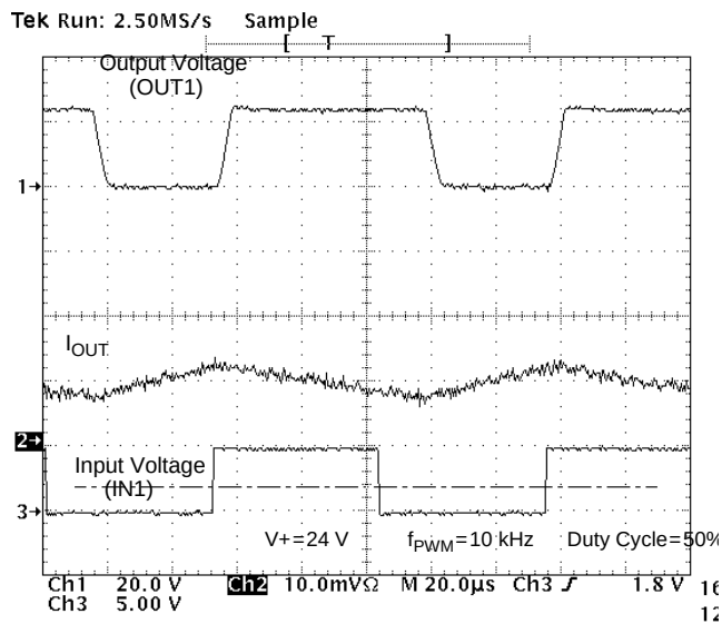
Figure 14. Output Voltage and Current vs. Input Voltage at V^+ = 24 \text{ V} , PWM Frequency of 10 kHz, and Duty Cycle of 50%
