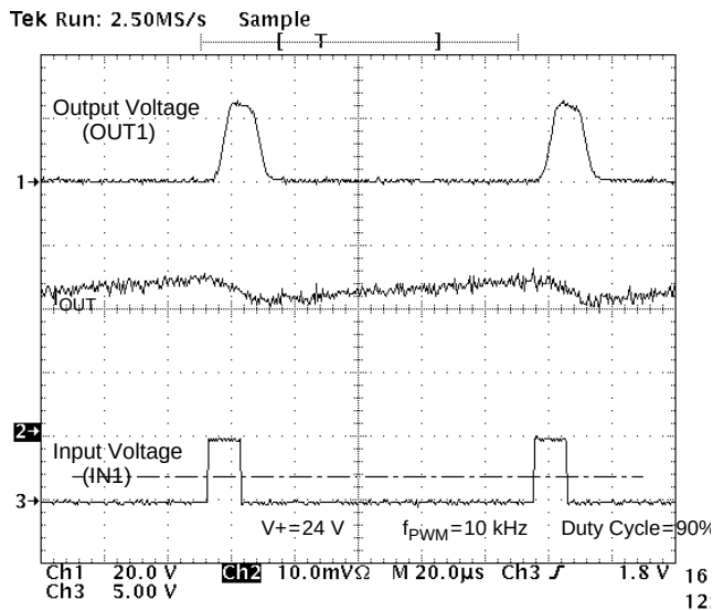
Figure 15. Output Voltage and Current vs. Input Voltage at V^+ = 24 \text{ V} , PWM Frequency of 10 kHz, and Duty Cycle of 90%
