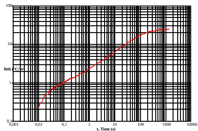
Figure 22. 33886 Thermal Response
