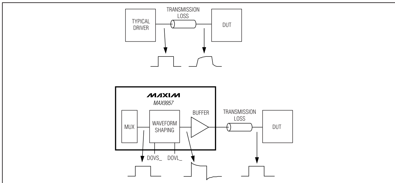
Figure 2. Waveform Shaping
