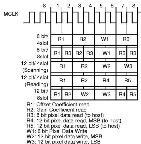
Figure 42: SRAM Access Modes
