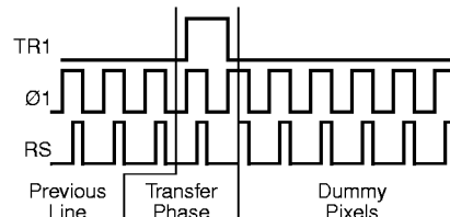
Figure 33: CIS TR1 Timing Mode 1
