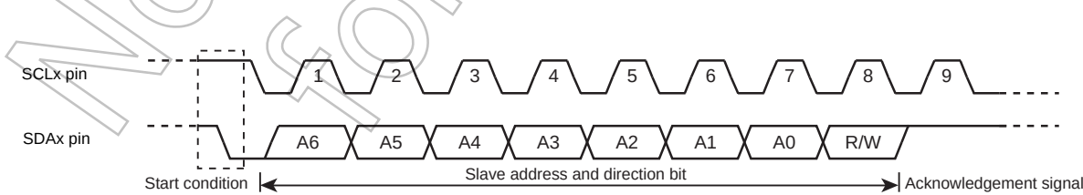
Figure 17-5 Generating the Start Condition and a Slave Address
