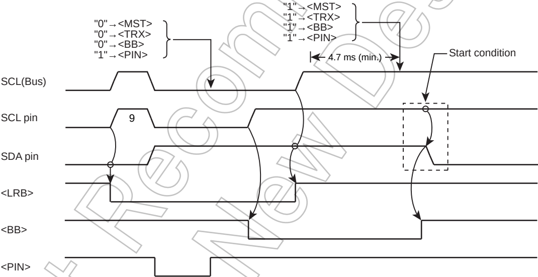
Figure 17-14 Timing Chart of Generating a Restart
