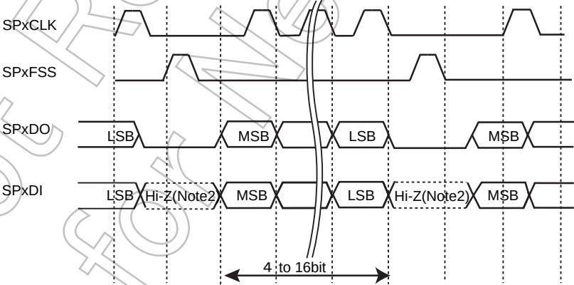
Figure 16-5 SPI frame format (continuous transfer, <SPO>="0" & <SPH>="0")
