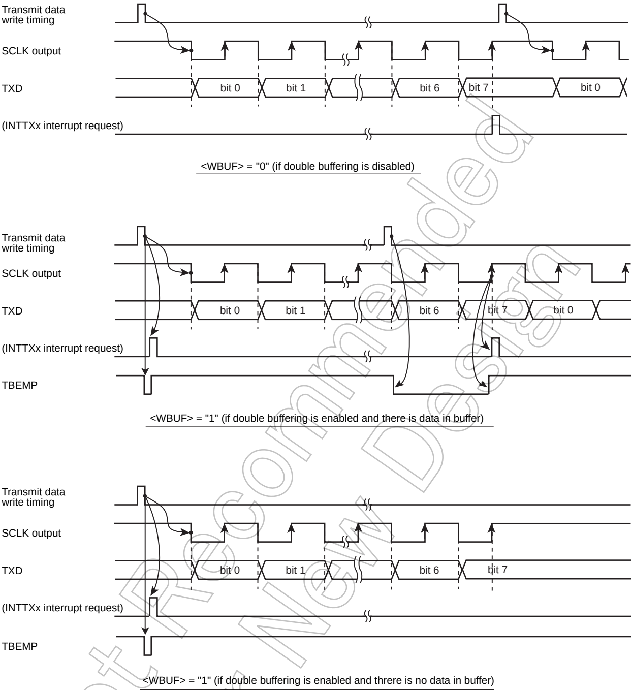
Figure 14-12 Transmit Operation in the I/O Interface Mode (SCLK Output Mode)
