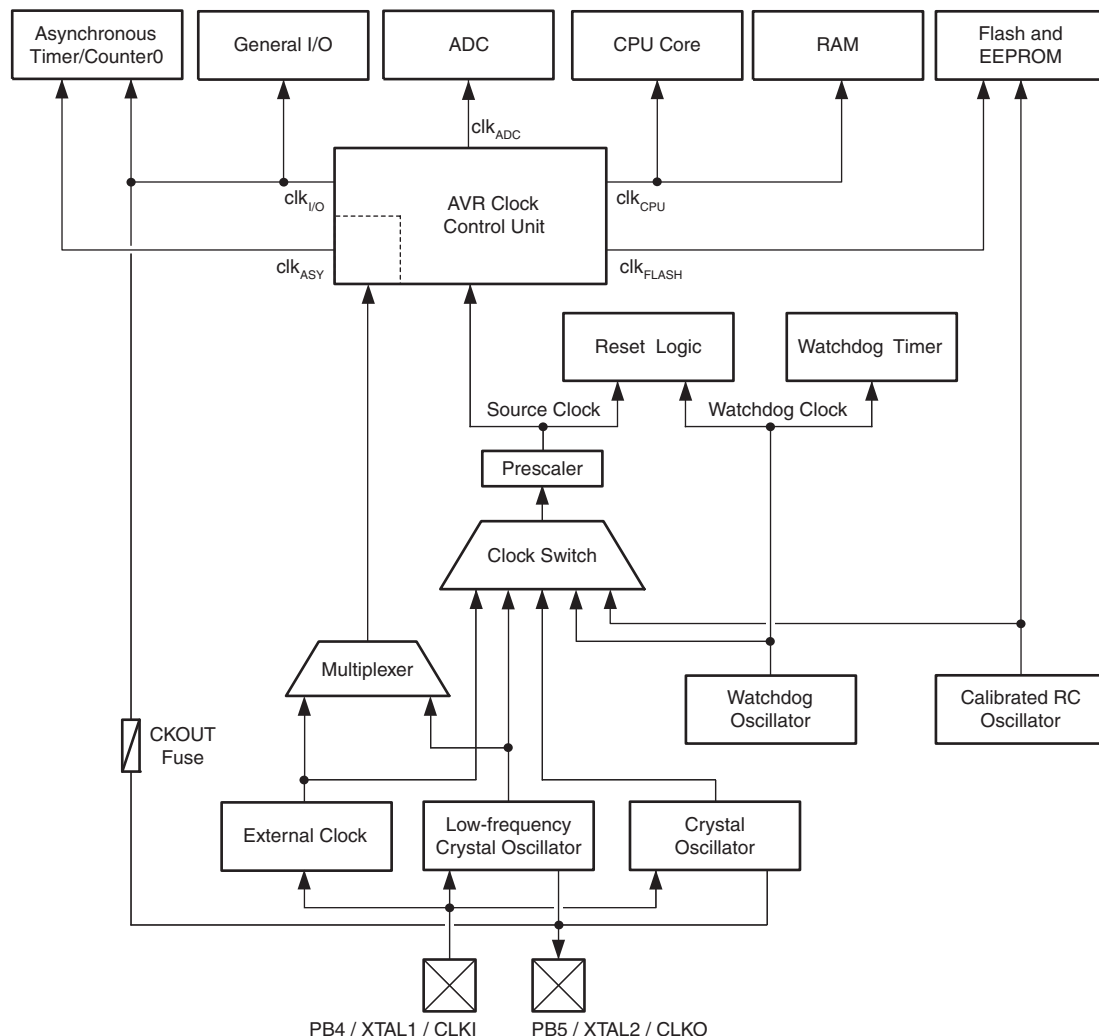
Figure 4-10. Clock Distribution
