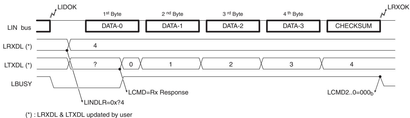
Figure 4-76. LIN2.1 - Rx Response - No Error
