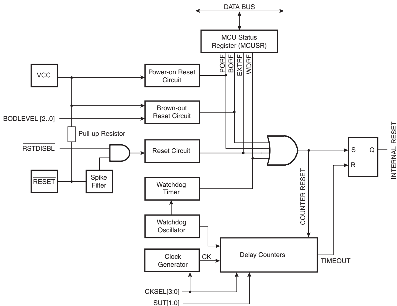
Figure 4-16. Reset Circuit
