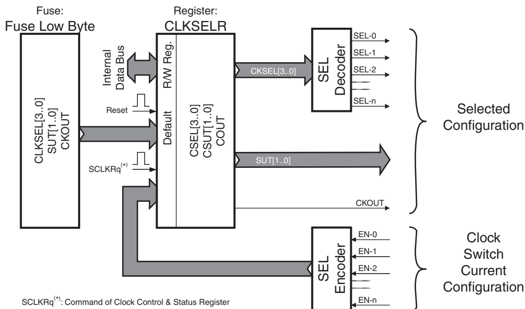
Figure 4-14. Fuses Substitution and Clock Source Selection
