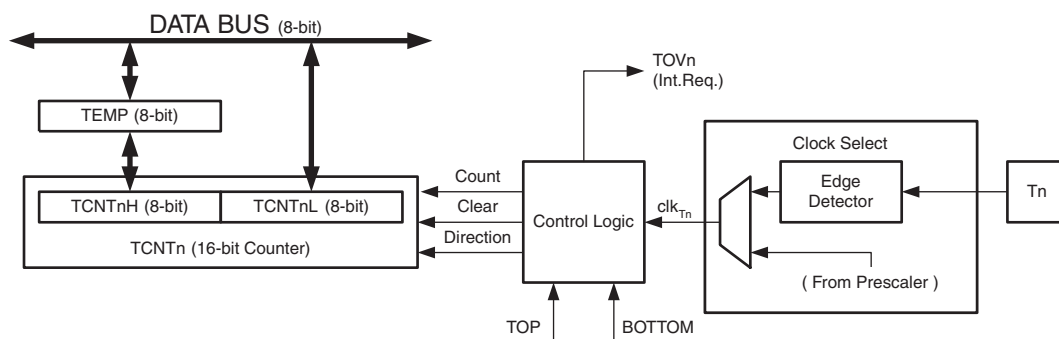
Figure 4-45. Counter Unit Block Diagram
