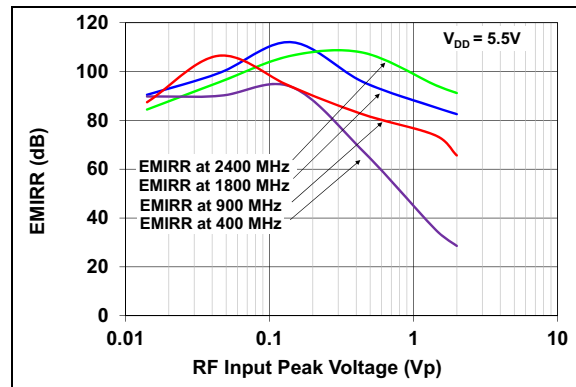
FIGURE 2-36: EMIRR vs. Input Voltage.
