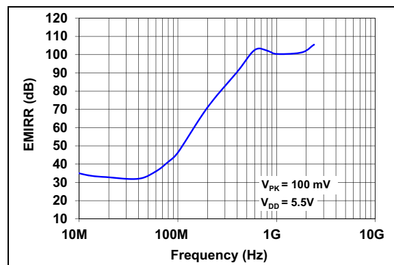
FIGURE 2-35: EMIRR vs. Frequency.
