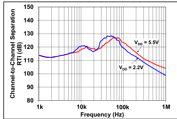
FIGURE 2-37: Channel-to-Channel Separation vs. Frequency.
