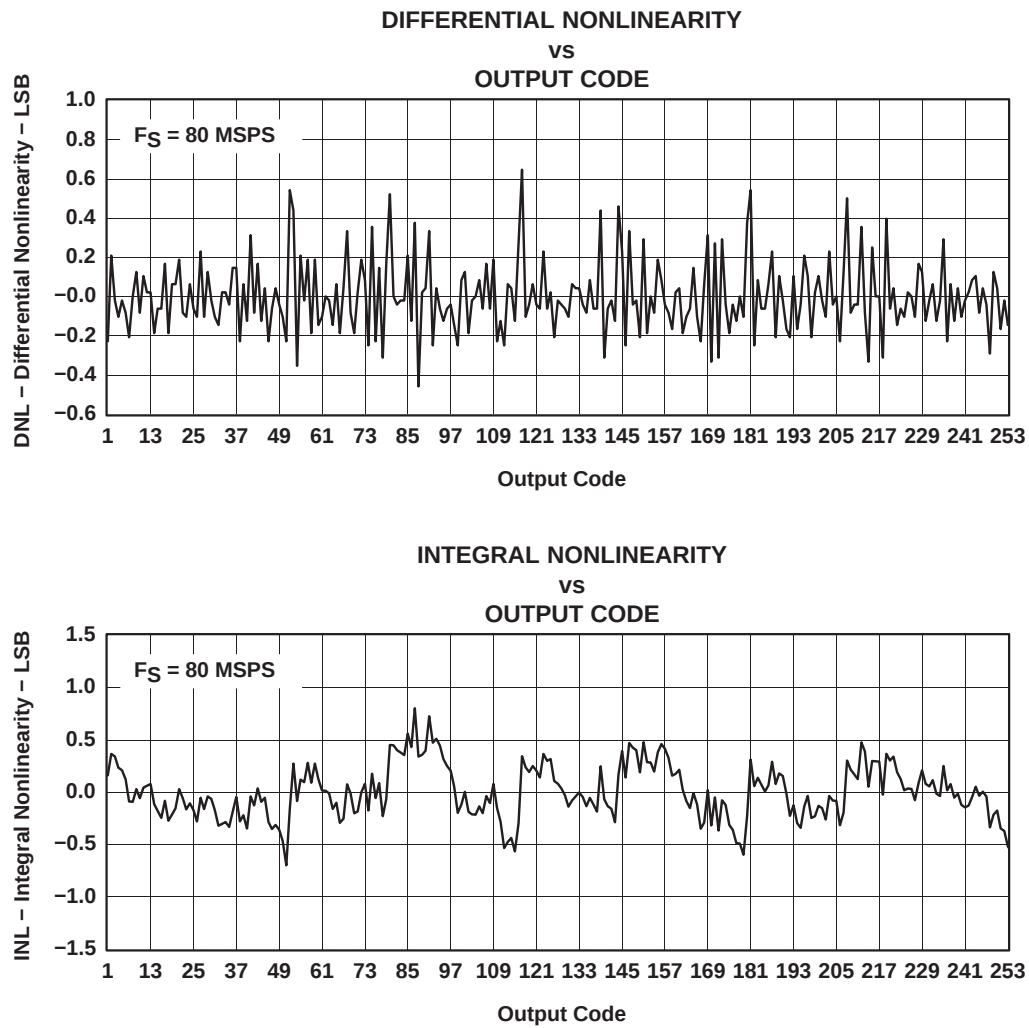
Figure 5–3. Linearity of AGY Channel at 80 MSPS (external clock)
