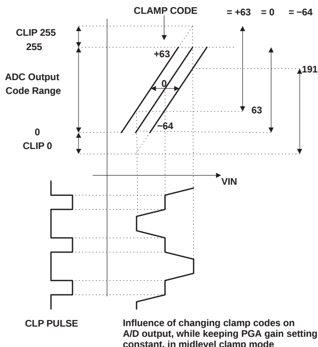
Figure 2-3. Mid-Level Clamping
