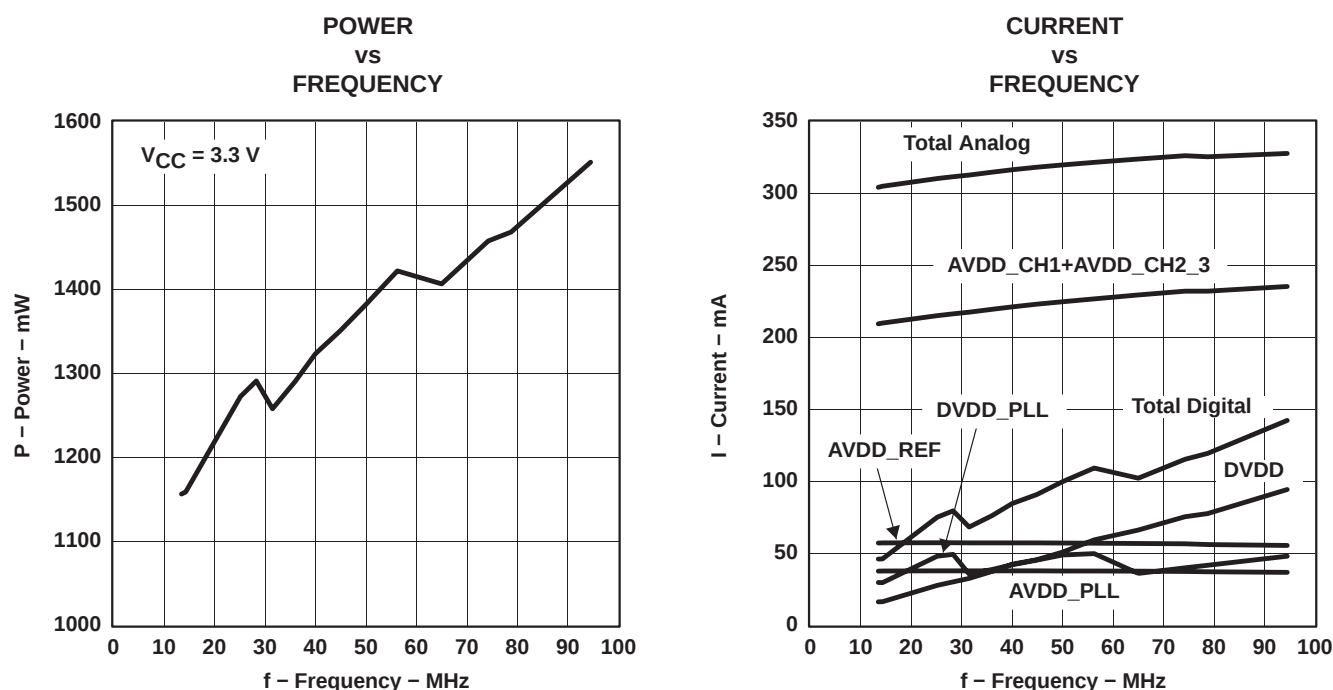
Figure 5-2. Power Consumption
