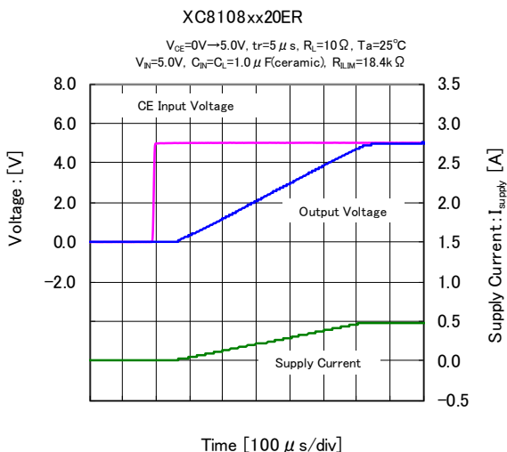
(16) turn-on Delay vs. Rise Time ( C_L=1.0\mu\text{F} )
