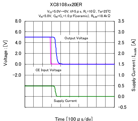
(17) turn-off Delay vs. Fall Time ( C_L=1.0\mu\text{F} )
