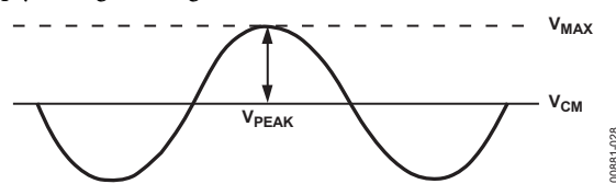
Figure 28. Common-Mode Definition
