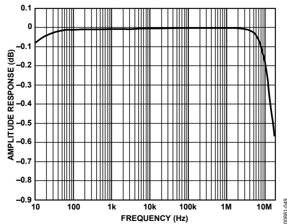
Figure 49. Amplitude Response vs. Frequency for Line Receiver
