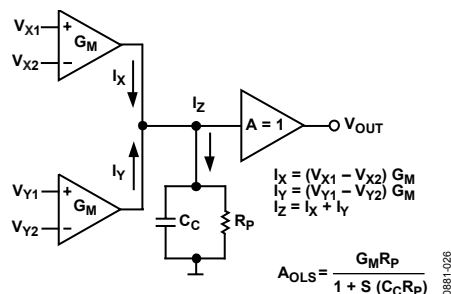
Figure 26. Topology Diagram
