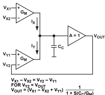
Figure 27. Closed-Loop Connection
