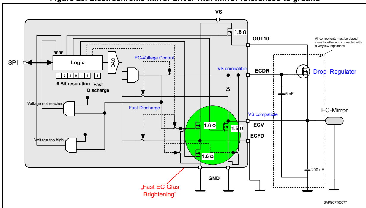
Figure 20. Electrochromic mirror driver with mirror referenced to ground
