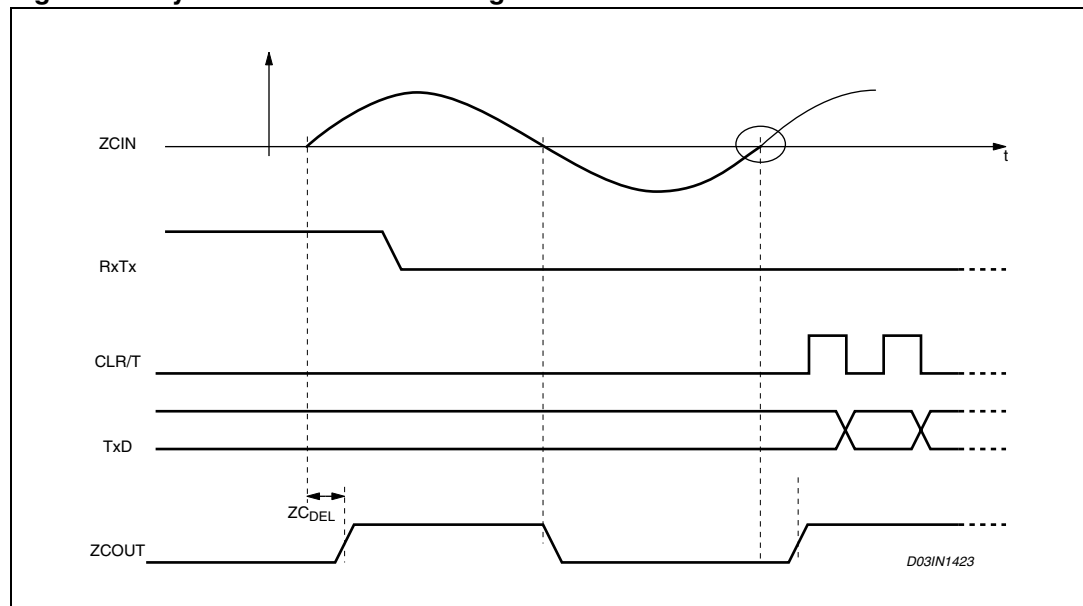
Figure 22. Synchronous zero-crossing transmission
