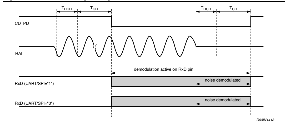
Figure 11. CD_PD timing during RX
