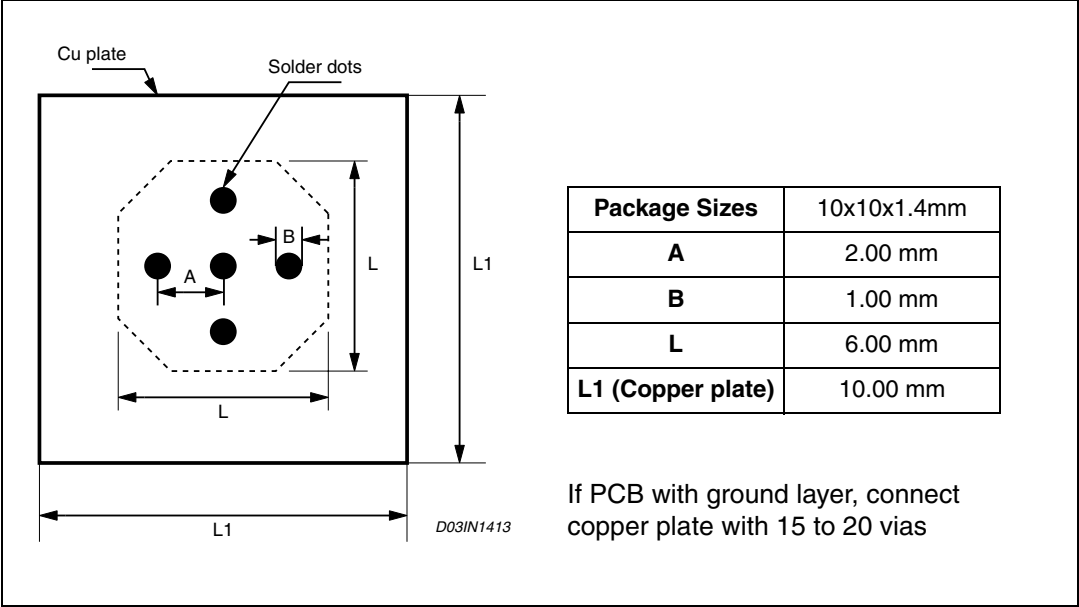
Figure 27. Soldering information
