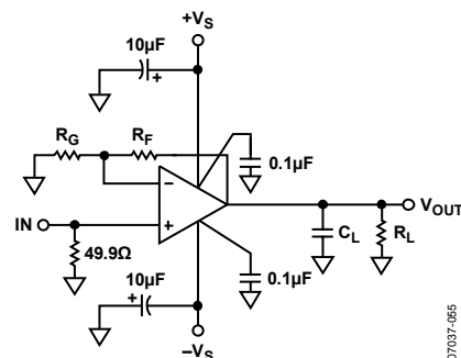
Figure 41. Typical Capacitive Load Configuration
