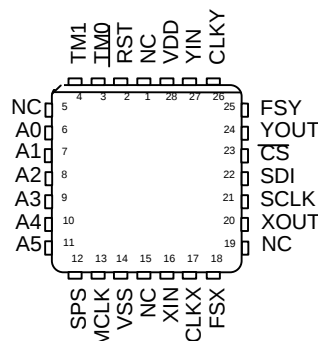
28-PIN PLCC
