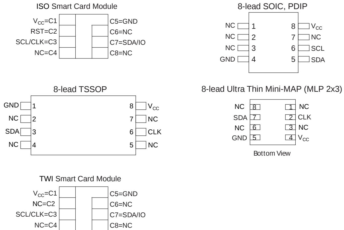
Figure 1. Pin Configuration
