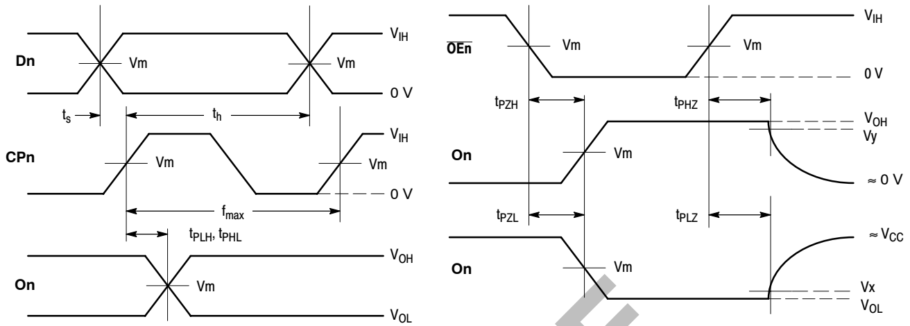
Figure 4. AC Waveforms
