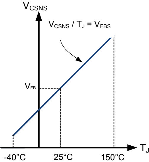
Figure 29. Temperature Reporting
