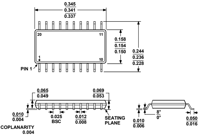
COMPLIANT TO JEDEC STANDARDS MO-137-AD Figure 11. 20-Lead Shrink Small Outline Package [QSOP] (RQ-20) Dimensions shown in inches
