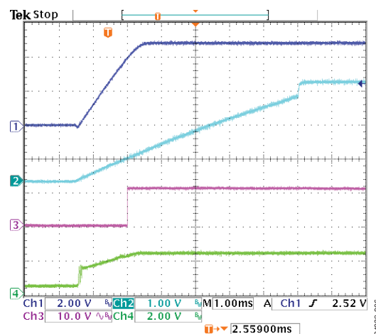
Figure 6. Typical Start-Up Waveforms Channel 1: CSREF, Channel 2: DELAY, Channel 3: PWRGD, Channel 4: COMP
