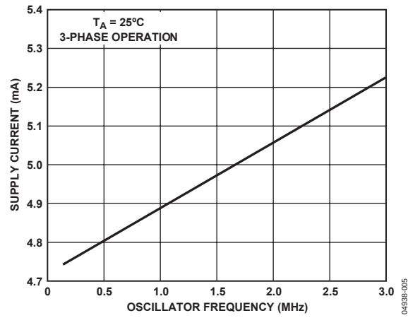
Figure 5. Supply Current vs. Oscillator Frequency
