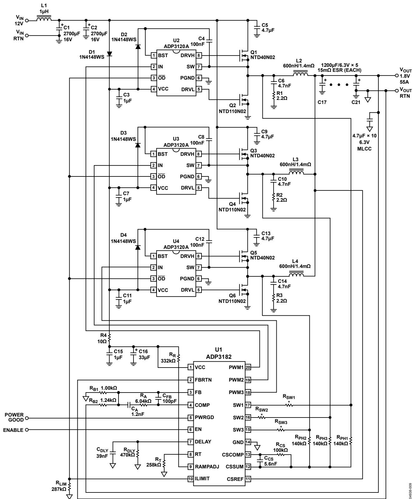
Figure 9. 1.8 V, 55 A Application Circuit
