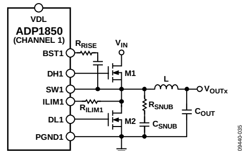
Figure 35. Application Circuit with a Snubber
