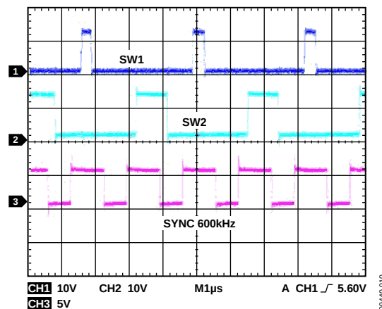
Figure 9. An Example of Synchronization, f_{\text{SYNC}} = 600 \text{ kHz}
