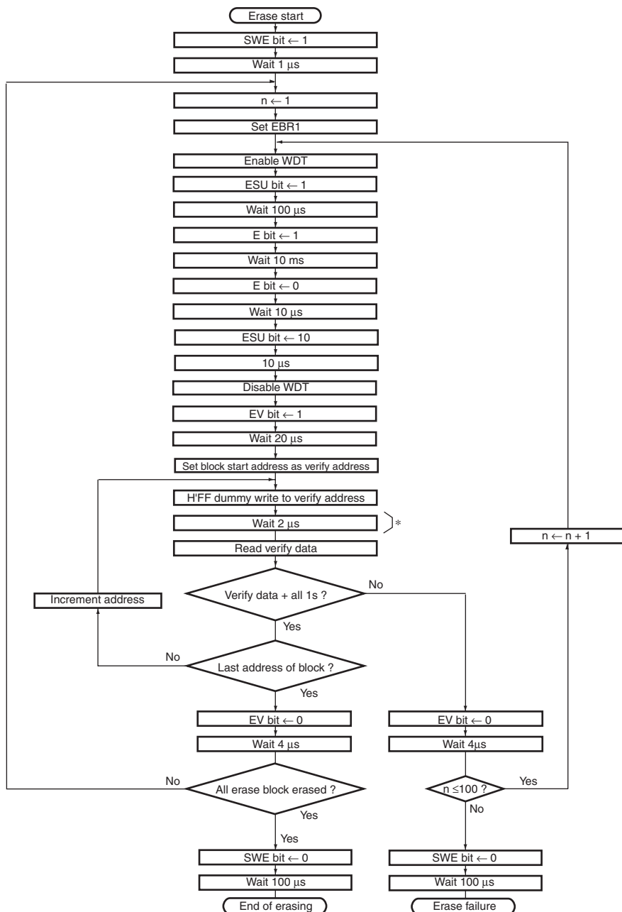
Figure 7.4 Erase/Eraser-Verify Flowchart
