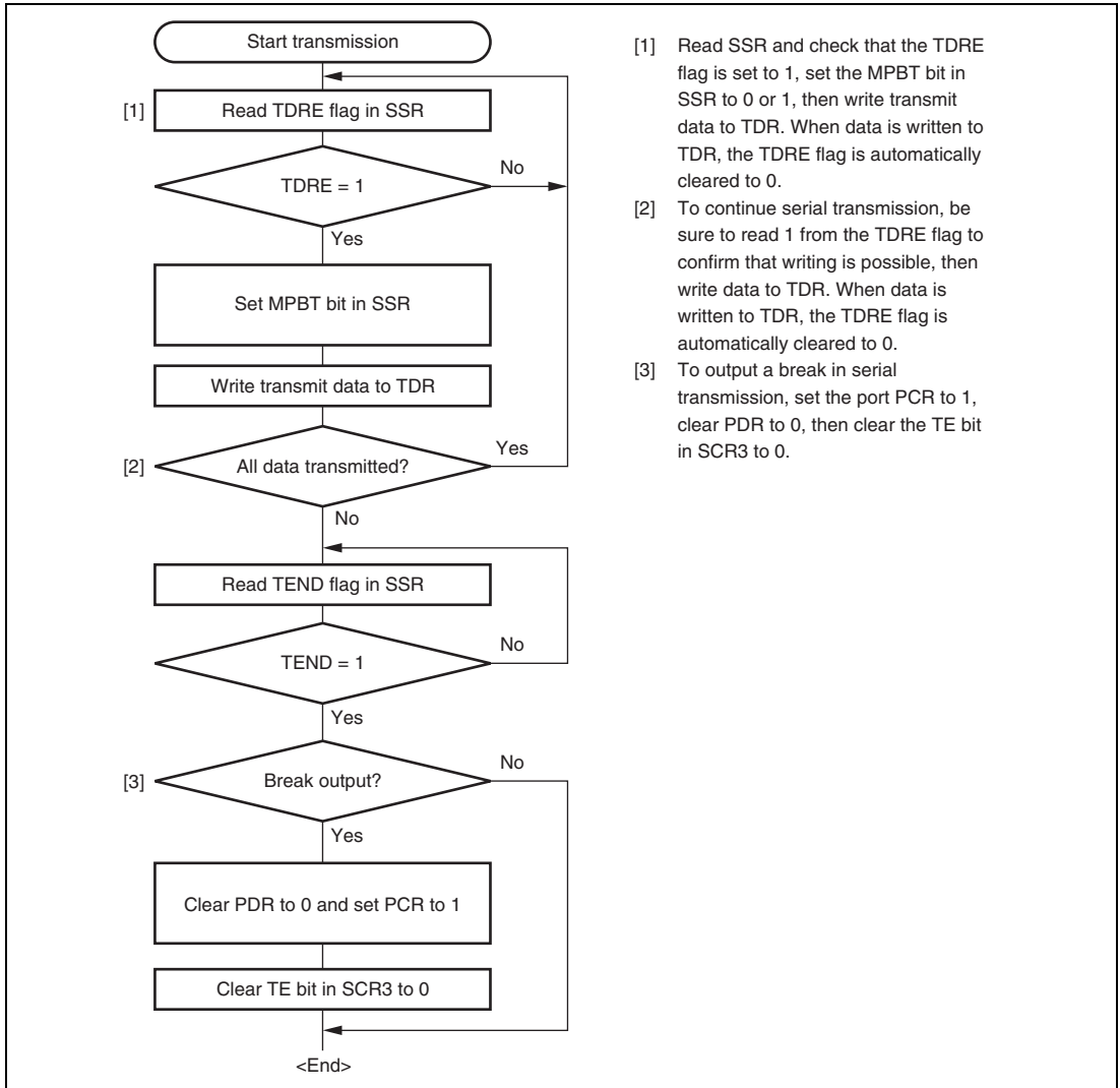
Figure 14.16 Sample Multiprocessor Serial Transmission Flowchart
