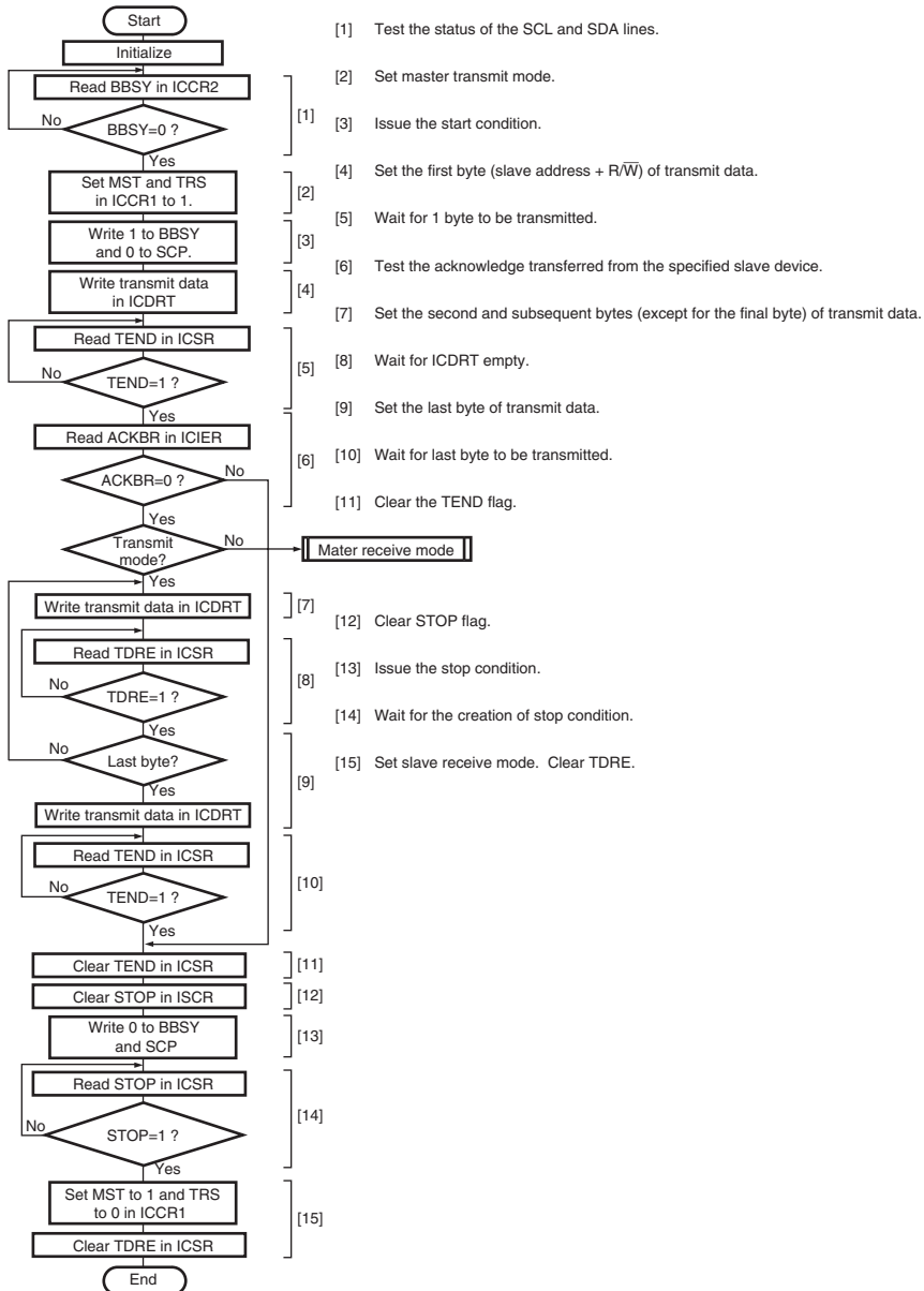
Figure 15.17 Sample Flowchart for Master Transmit Mode
