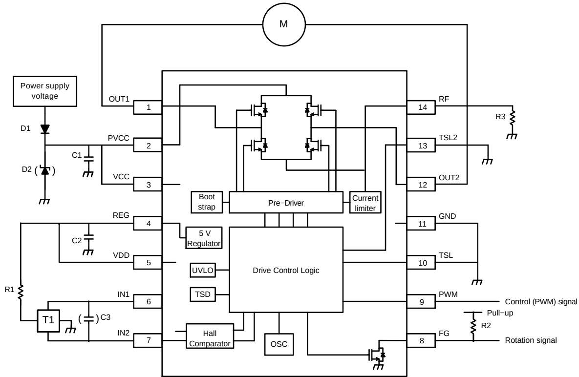
Figure 1. Application diagram
