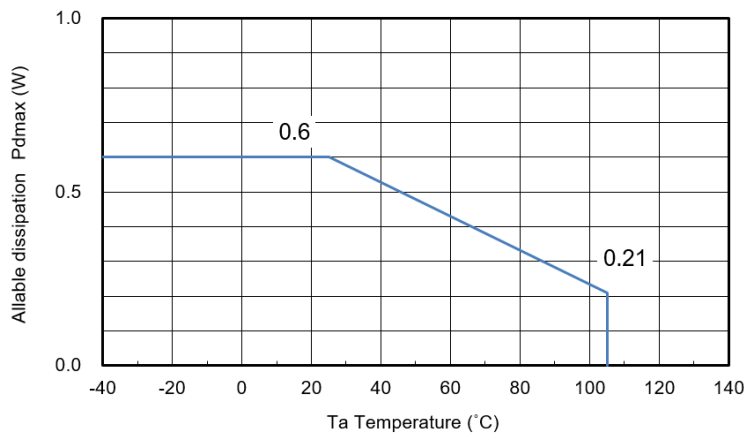
Figure 2. Power Dissipation vs. Ambient Temperature Characteristics
