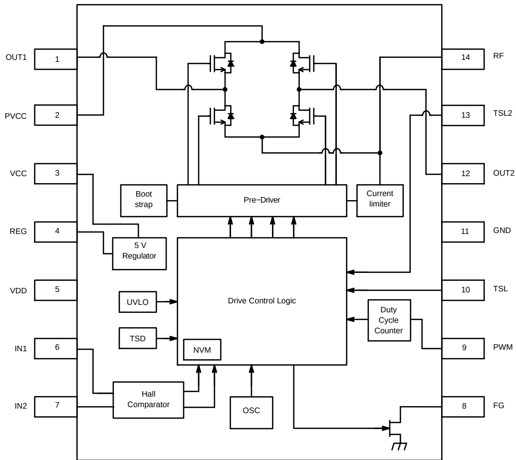
Figure 3. Block Diagram
