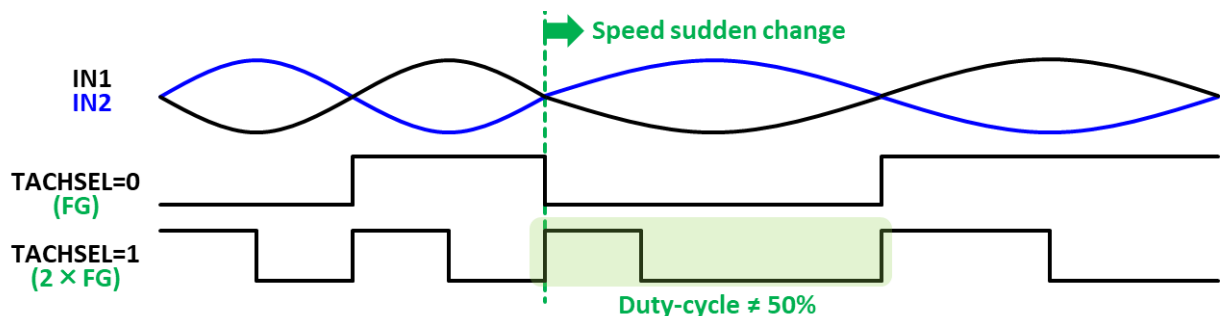
Figure 17. FG Duty-cycle
