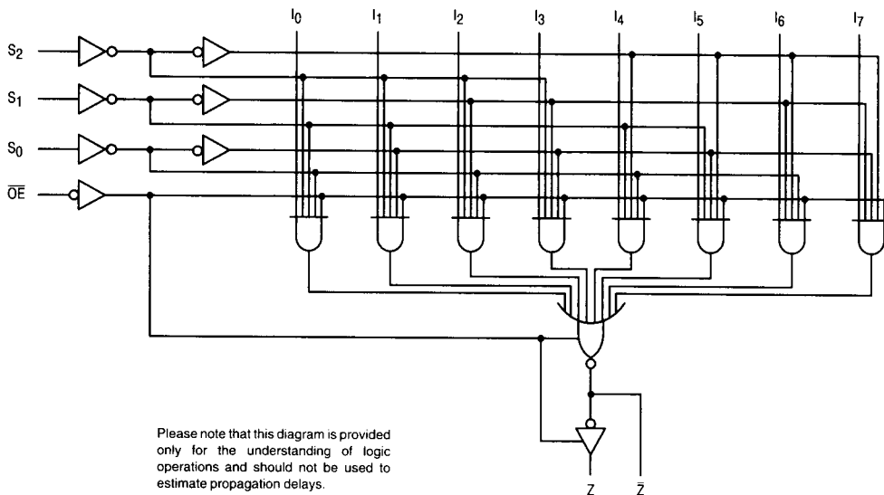
LOGIC DIAGRAM
