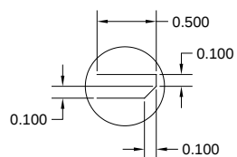
DETAIL A PIN #1 TERMINAL SCALE: 2X
