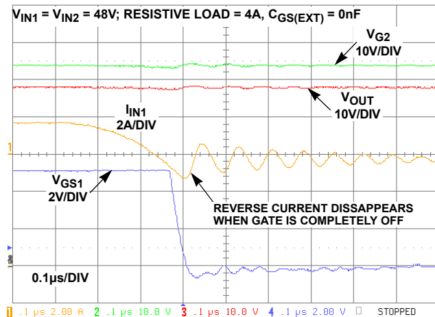
FIGURE 21. FAST SPEED TURN-OFF (MOSFET WITH Q TOT = 8.4nC)
