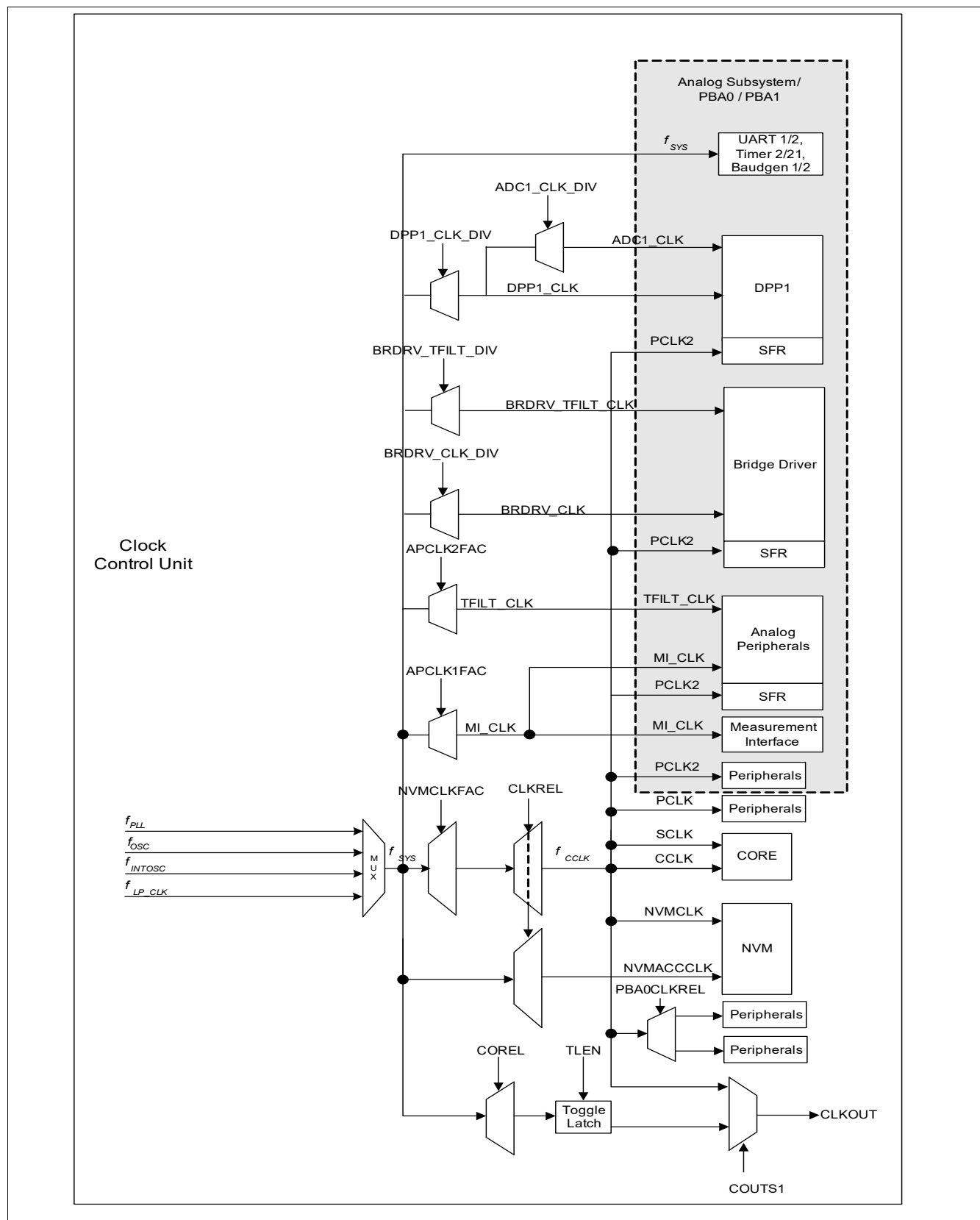
Figure 13 Clock Generation from f_{\text{sys}} ; CLKOUT Generation
