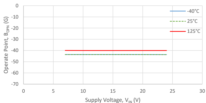
Operate Point, North ( B_{OPN} v. V_{IN} )
