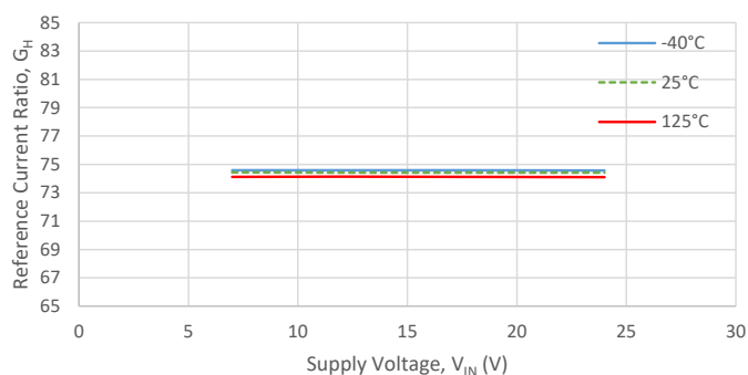
Reference Current Ratio ( G_H v. V_{IN} )
