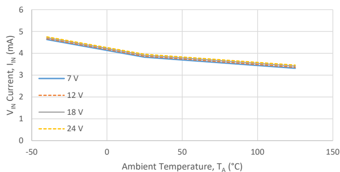
V_{IN} Active Current ( I_{IN(ACT)} v. T_A )
