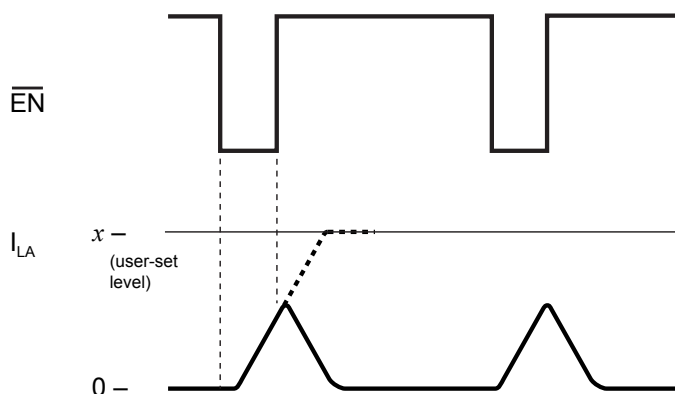
Figure 10: High PWM Duty Cycle
