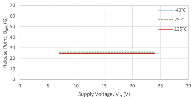
Release Point, South ( B_{RPS} v. V_{IN} )
