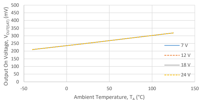
Output On Voltage ( V_{OUT(SAT)} v. T_A )
