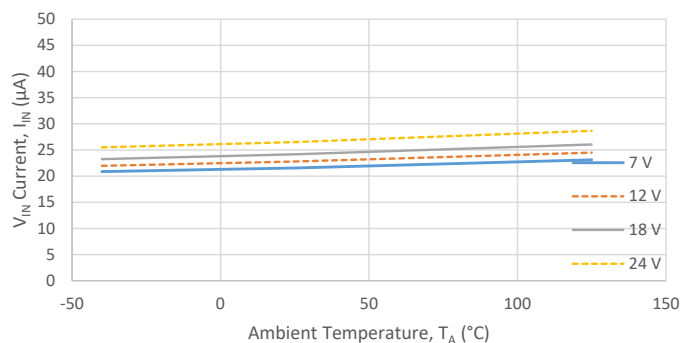
V_{IN} Average Current ( I_{IN(AVG)} v. T_A )
