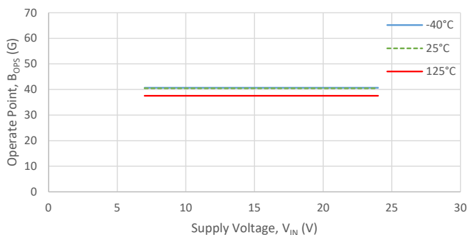
Operate Point, South ( B_{OPS} v. V_{IN} )
