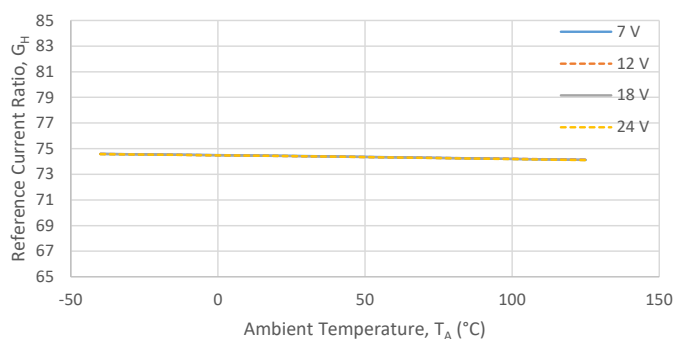
Reference Current Ratio ( G_H v. T_A )
