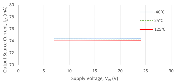
Output Source Current ( I_{LA} v. V_{IN} )
