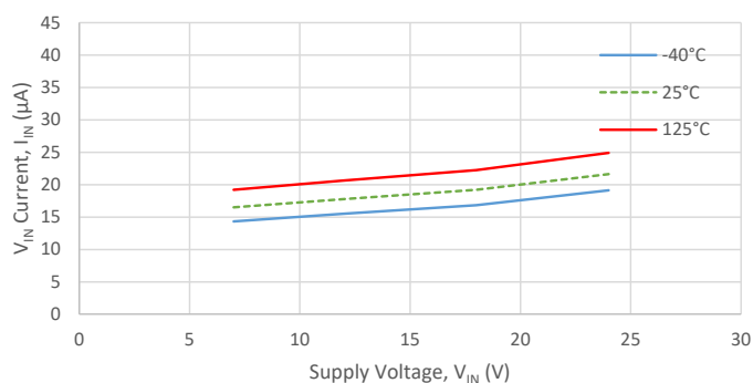
V_{IN} Quiescent Current ( I_{INQ} v. V_{IN} )
