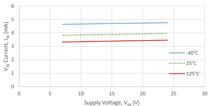
V_{IN} Active Current ( I_{IN(ACT)} v. V_{IN} )
