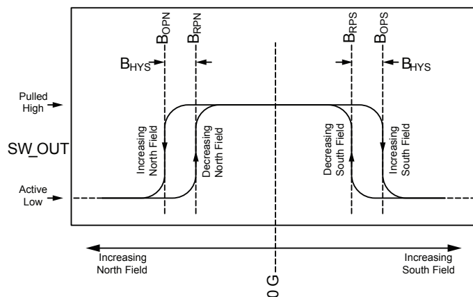
Figure 3: Hall Switch Output ( \overline{SW} ) State versus Magnetic Field (POL = float)
