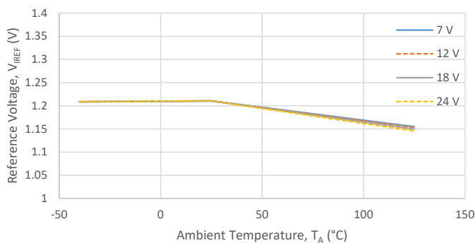
Reference Voltage ( V_{REF} v. T_A )
