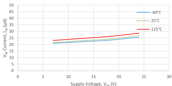
V_{IN} Average Current ( I_{IN(AVG)} v. V_{IN} )
