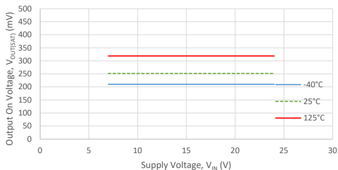
Output On Voltage ( V_{OUT(SAT)} v. V_{IN} )
