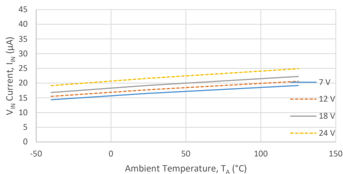
V_{IN} Quiescent Current ( I_{INQ} v. T_A )
