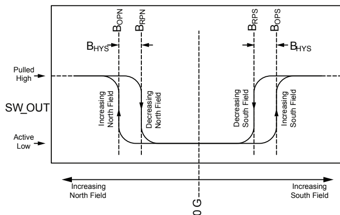
Figure 4: Hall Switch Output ( \overline{SW} ) State versus Magnetic Field (POL = GND)
