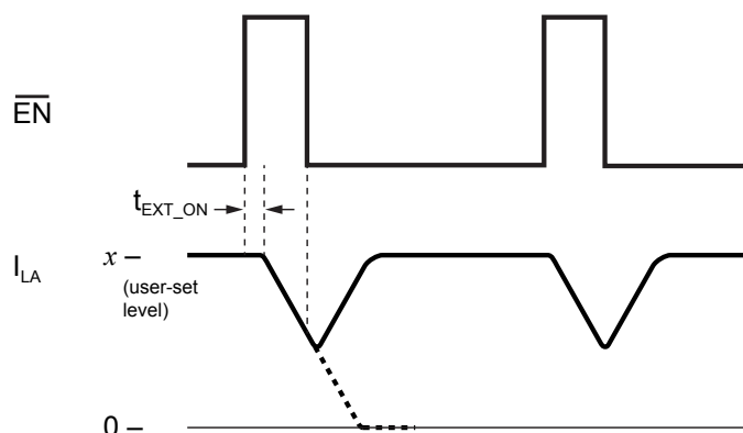
Figure 9: Low PWM Duty Cycle
