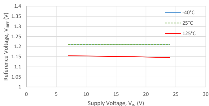
Reference Voltage ( V_{REF} v. V_{IN} )
