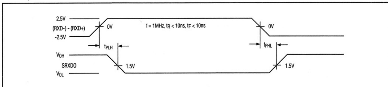
Figure 10. Differential Receiver Switching Times
