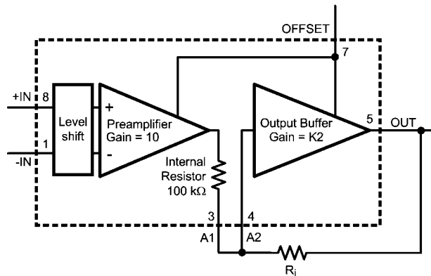
FIGURE 5. Increase Gain
