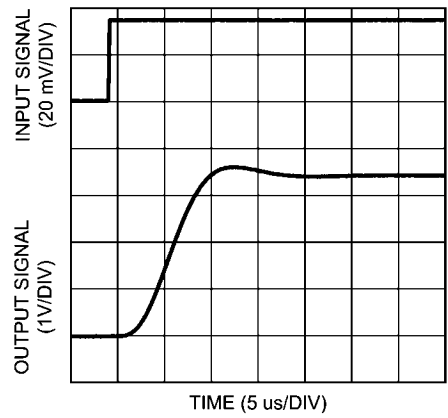
Settling Time (Rising Edge) at V_S = 5V LMP8603
