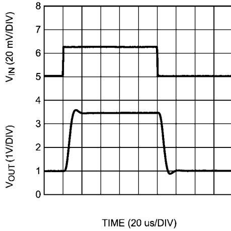
Step Response at V_S = 3.3V R_L = 10k\Omega LMP8603
