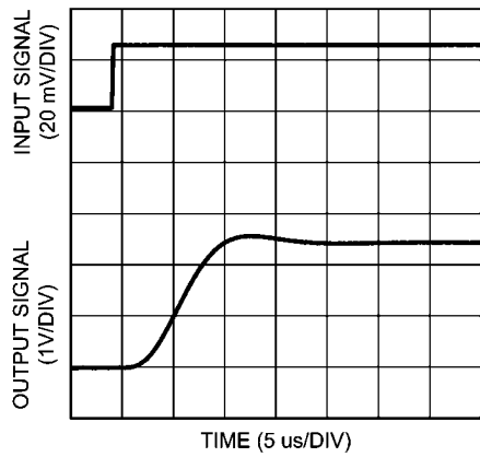
Settling Time (Rising Edge) at V_S = 3.3V LMP8603
