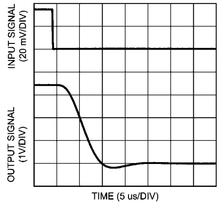
Settling Time (Falling Edge) at V_S = 5V LMP8603
