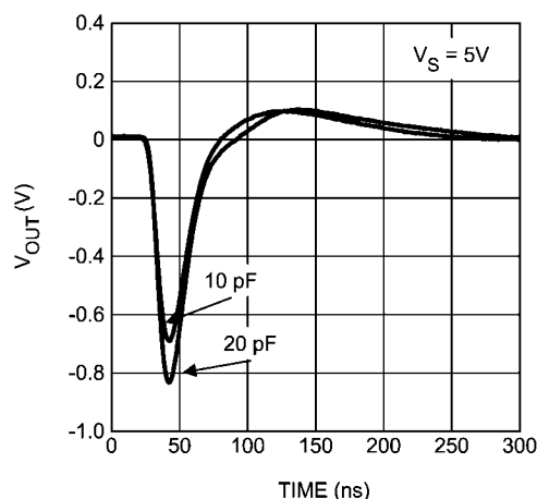
FIGURE 8. Capacitive Load Response at 5.0V
