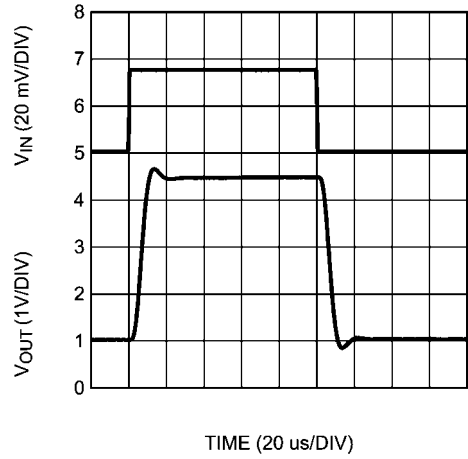
Step Response at V_S = 5V R_L = 10k\Omega LMP8603
