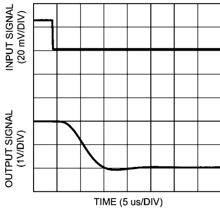
Settling Time (Falling Edge) at V_S = 3.3V LMP8603
