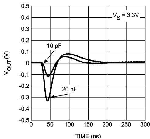
FIGURE 7. Capacitive Load Response at 3.3V
