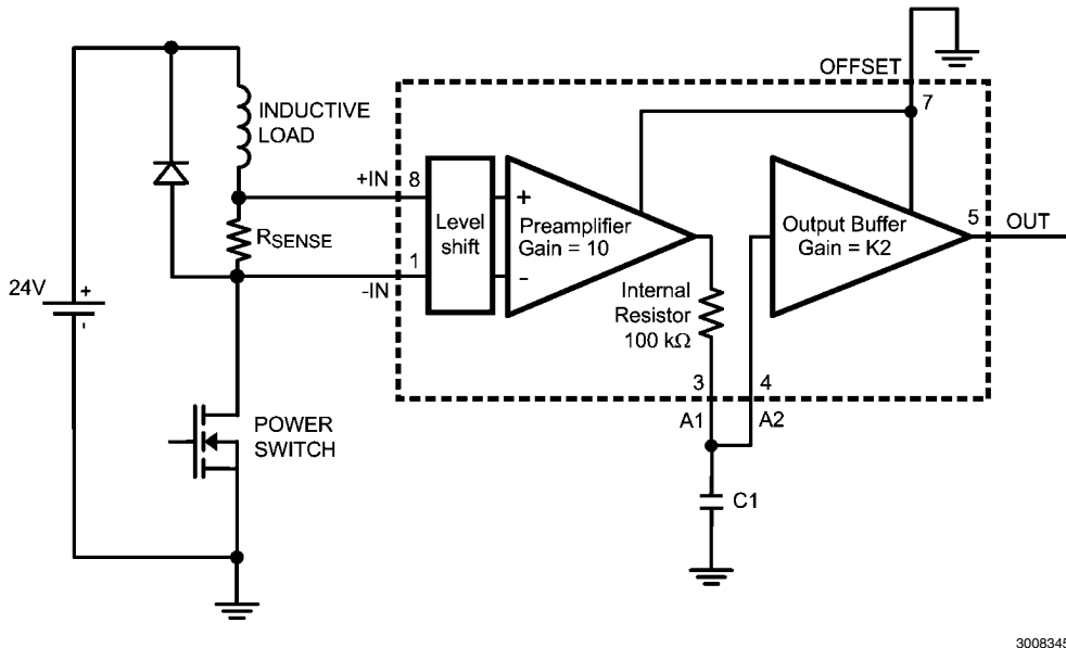
FIGURE 10. Low Side Current Sensing Application with Large Common Mode Transients
