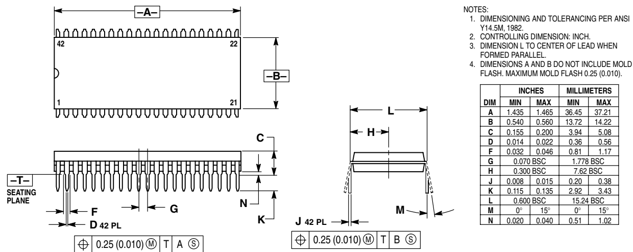
Figure 25-3. 42-Pin SDIP (Case #858)
