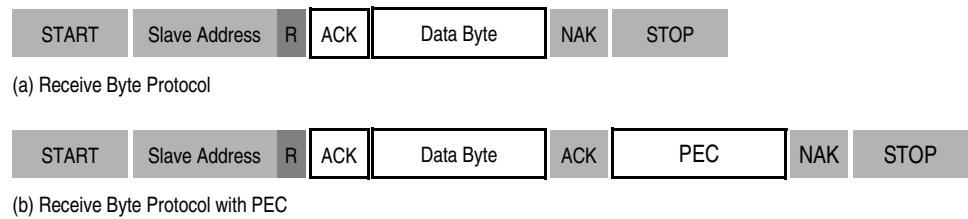
Figure 16-15. Receive Byte
