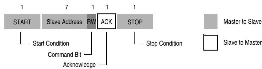
Figure 16-13. Quick Command
