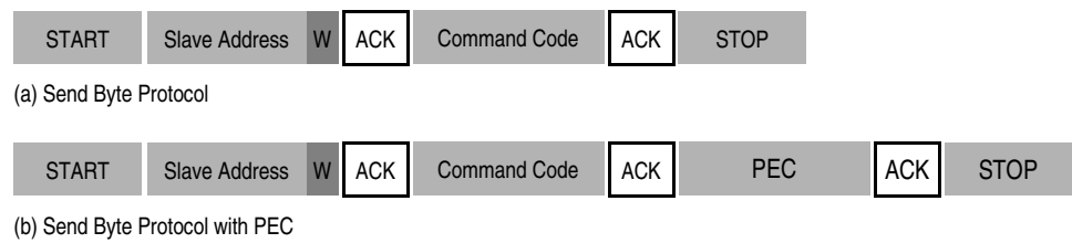
Figure 16-14. Send Byte
