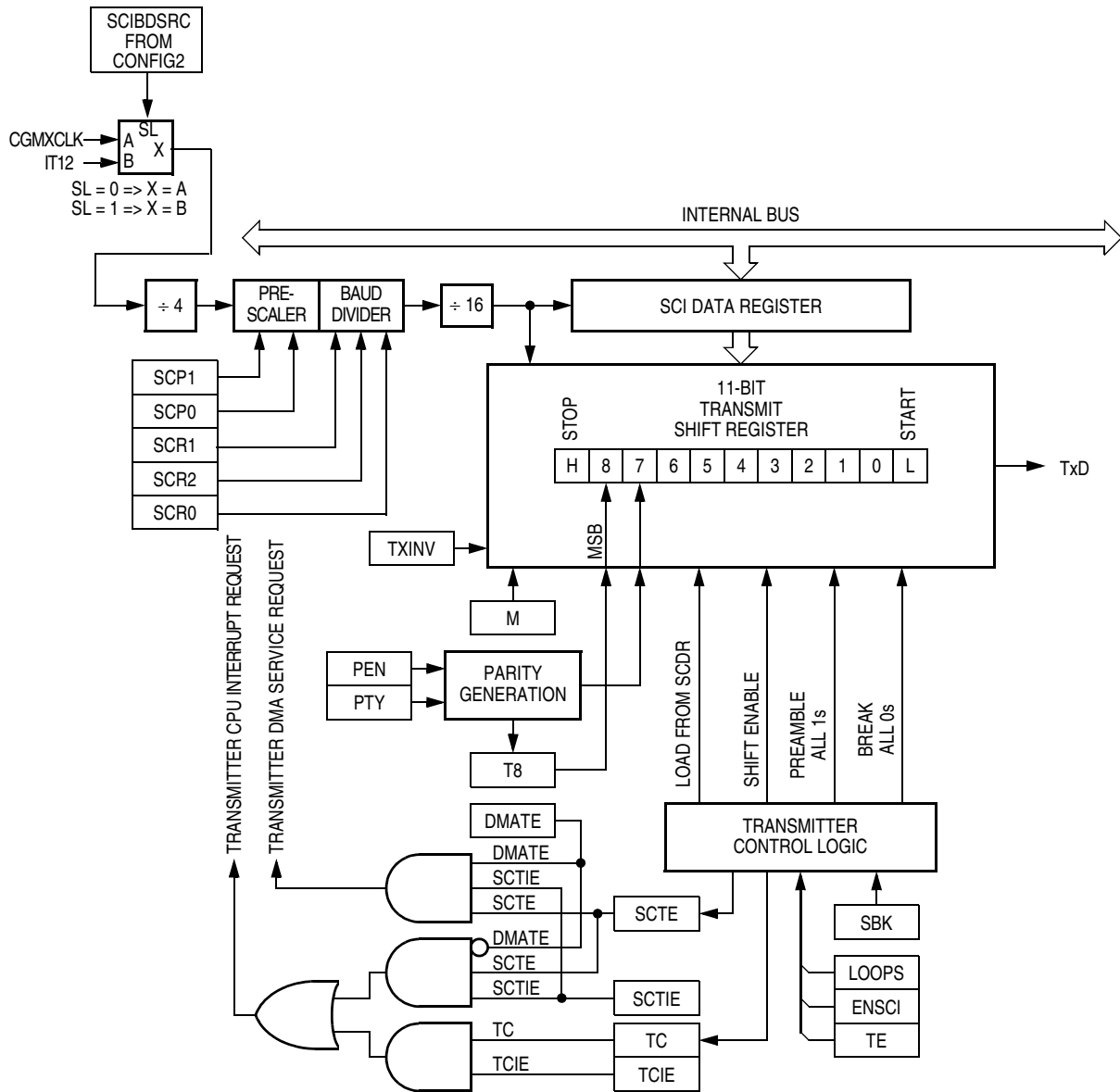
Figure 13-4. SCI Transmitter
