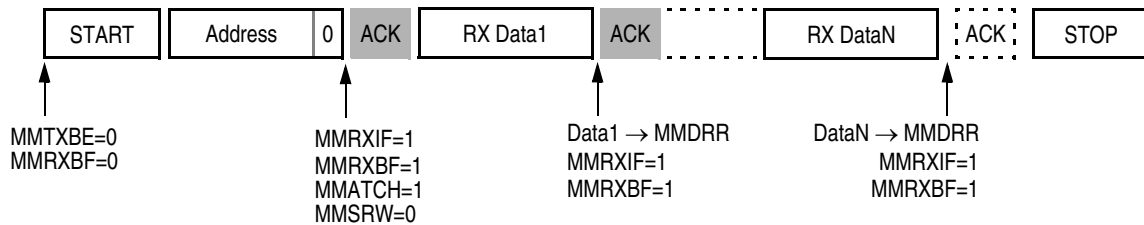
Figure 16-12. Data Transfer Sequences for Master/Slave Transmit/Receive Modes
