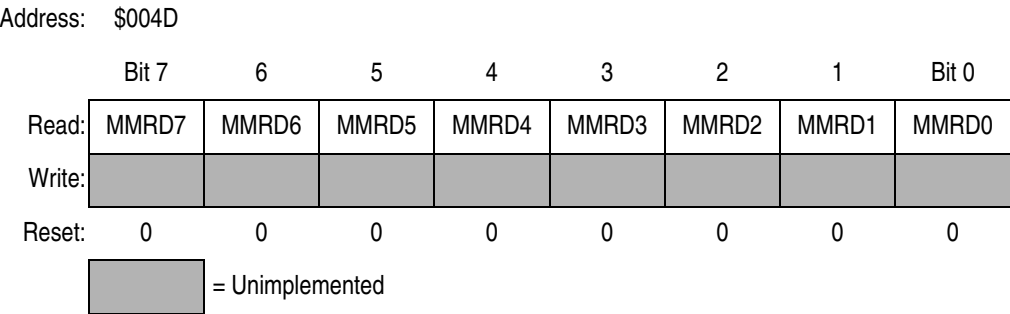
Figure 16-9. MMIIC Data Receive Register (MMDRR)
