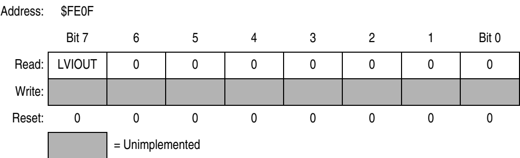
Figure 22-3. LVI Status Register
