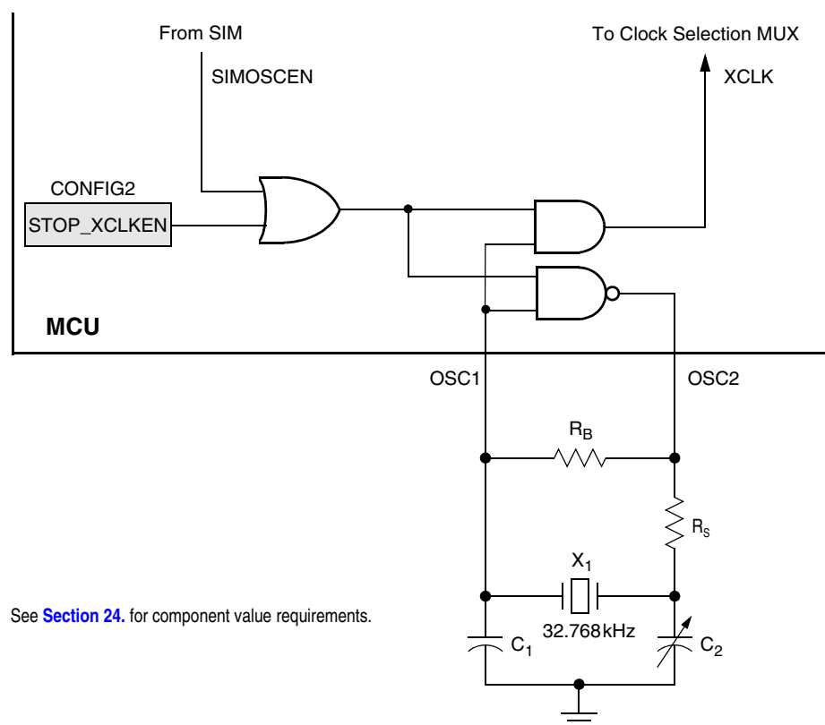
Figure 7-6. Crystal Oscillator
