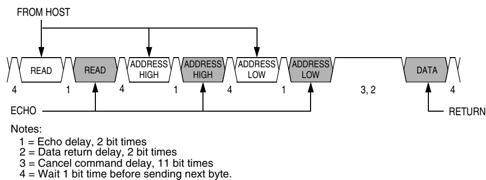
Figure 10-5. Read Transaction
