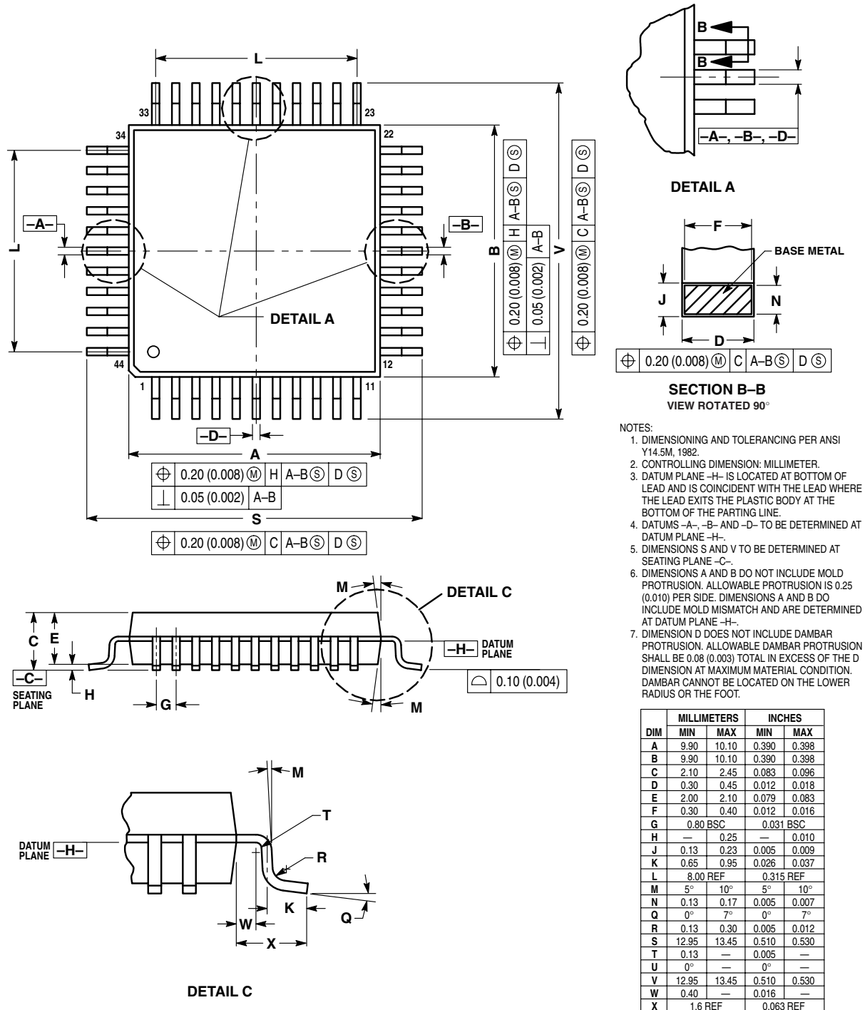
Figure 25-2. 44-Pin QFP (Case #824A)
