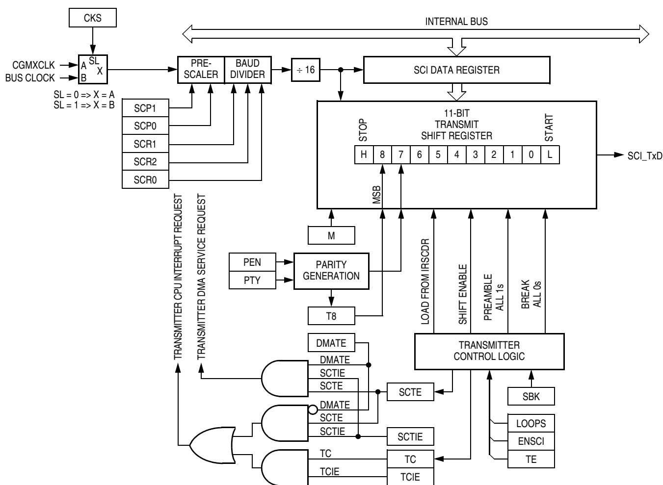
Figure 14-7. SCI Transmitter
