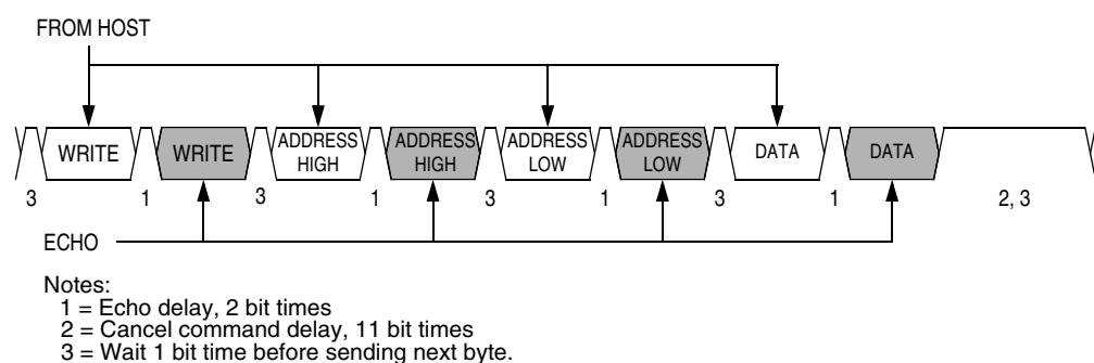
Figure 10-6. Write Transaction
