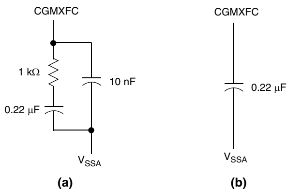
Figure 8-10. PLL Filter
