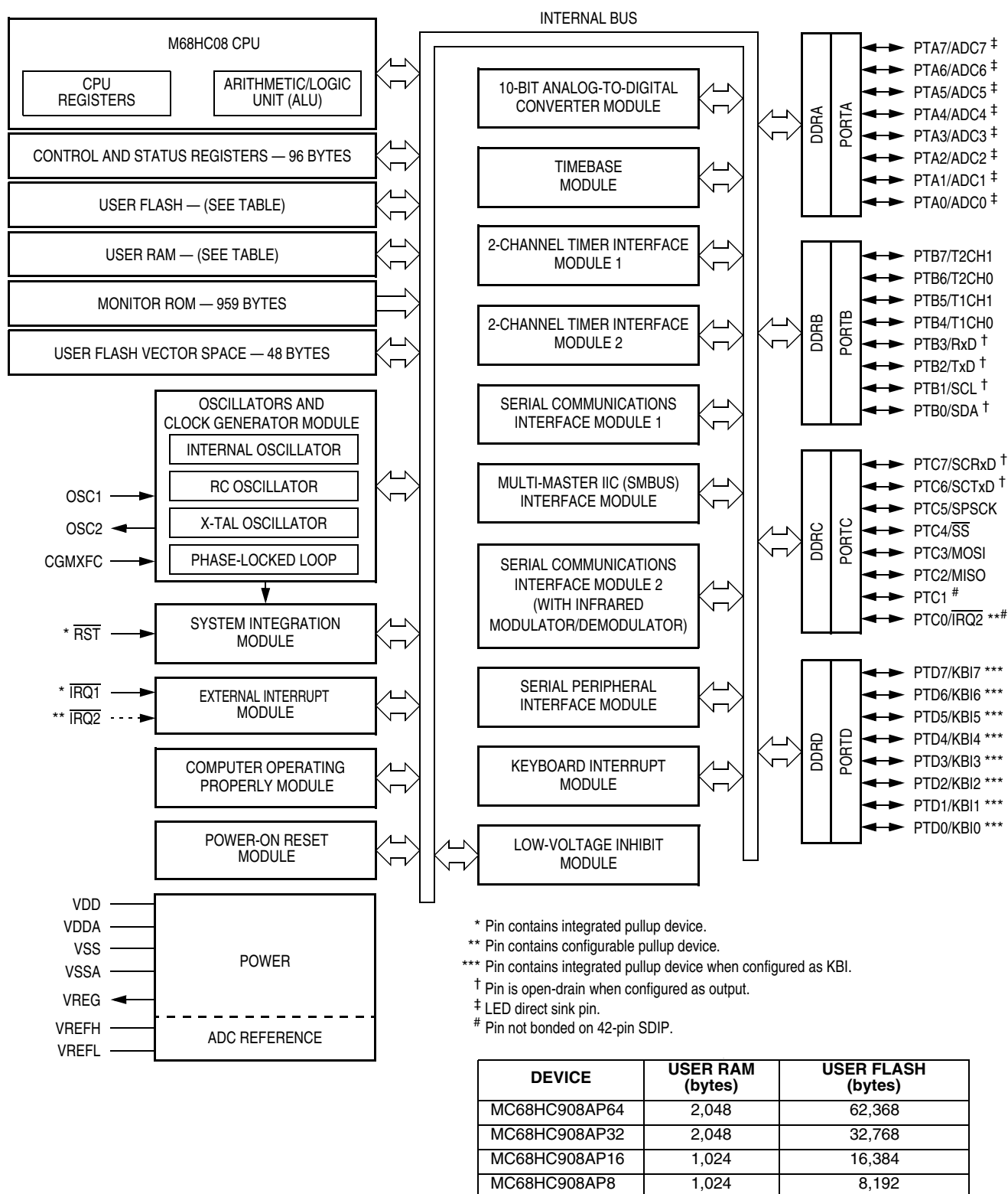
Figure 1-1. MC68HC908AP64 Block Diagram
