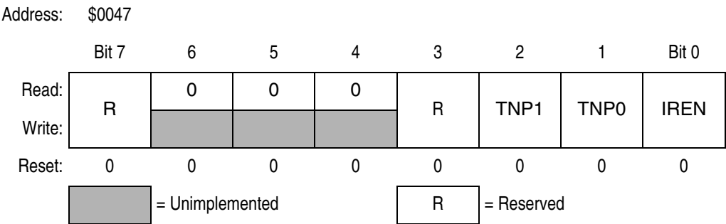
Figure 14-20. IRSCI Infrared Control Register (IRSCIRCR)
