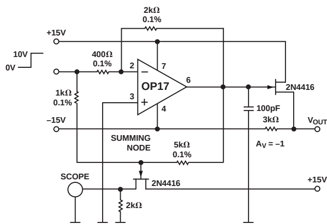
Figure 6. OP17 Settling Time Test Circuit
