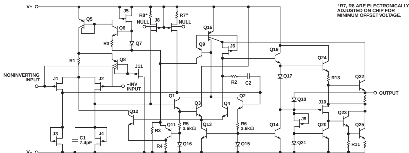
Figure 1. Simplified Schematic
