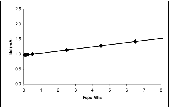
Figure 134. Typical I_{DD} in Slow-wait vs. f_{CPU}
