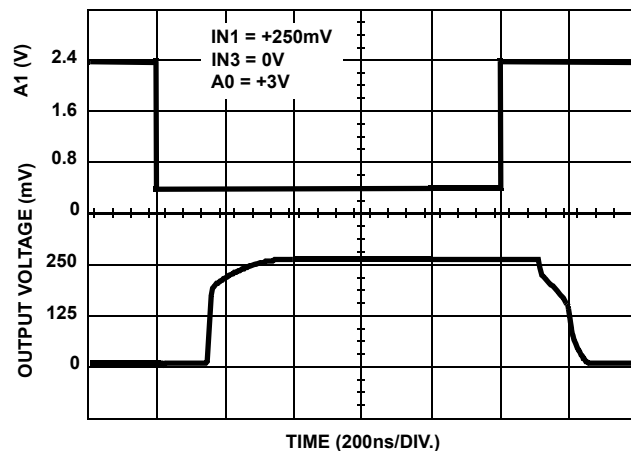
FIGURE 4. CHANNEL-TO-CHANNEL SWITCHING RESPONSE
