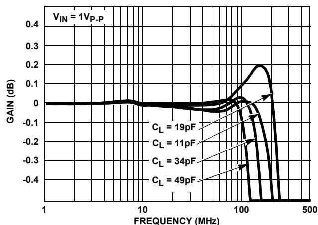
FIGURE 6. GAIN FLATNESS
